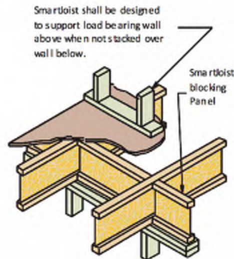
TYPICAL JOIST BLOCKING DETAIL nts
