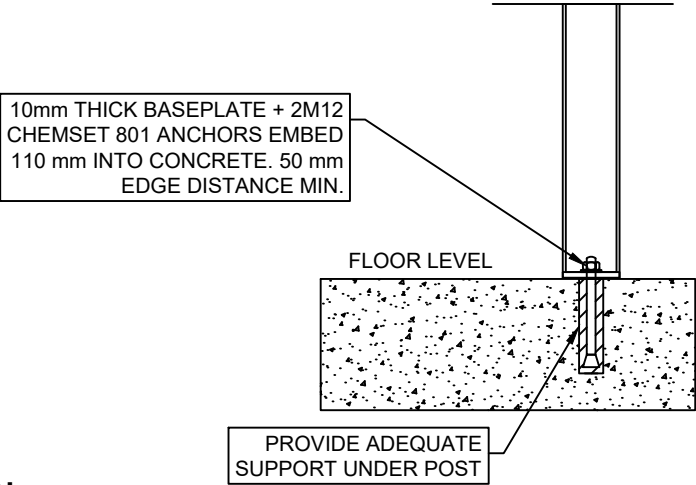
TYPICAL BASE PLATE CONNECTION DETAIL scale1 :10
