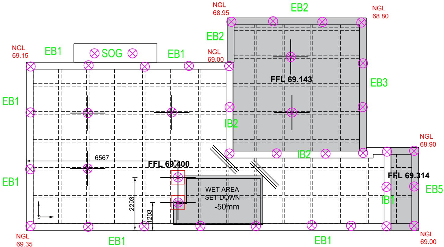
SLAB AND FOOTING PLAN scale 1:100
