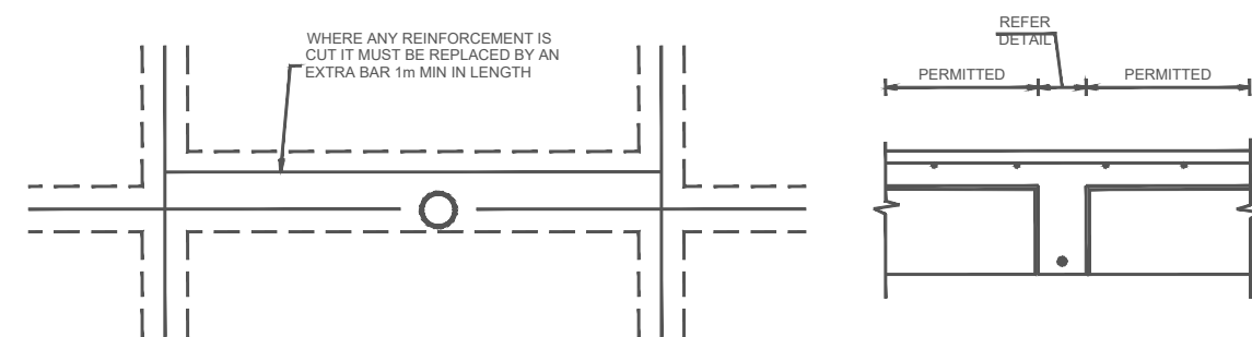
TYPICAL INTERNAL RIB VERTICAL PIPE PENETRATION DETAIL NTS
