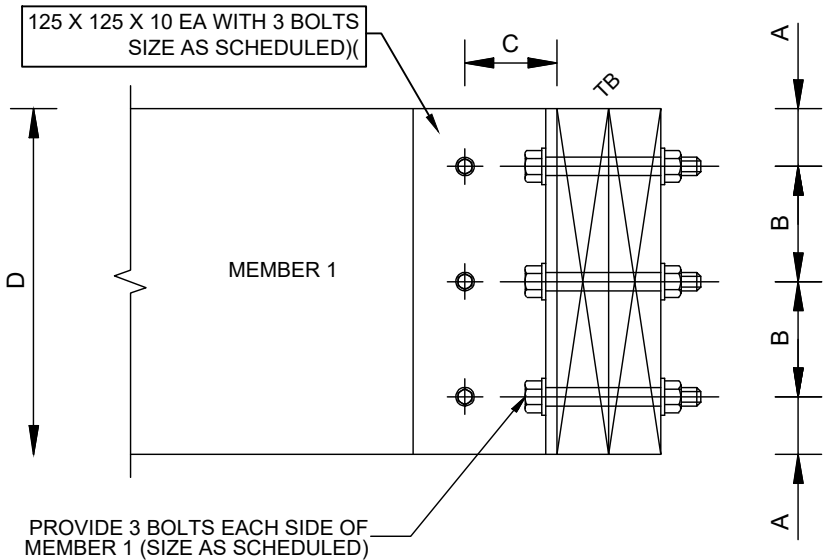
TYPICAL TIMBER BEAM TO TIMBER BEAM CONNECTION DETAIL
