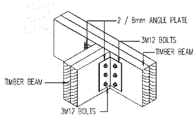
TIMBER BEAM - TIMBER BEAM CONNECTION not to scale
