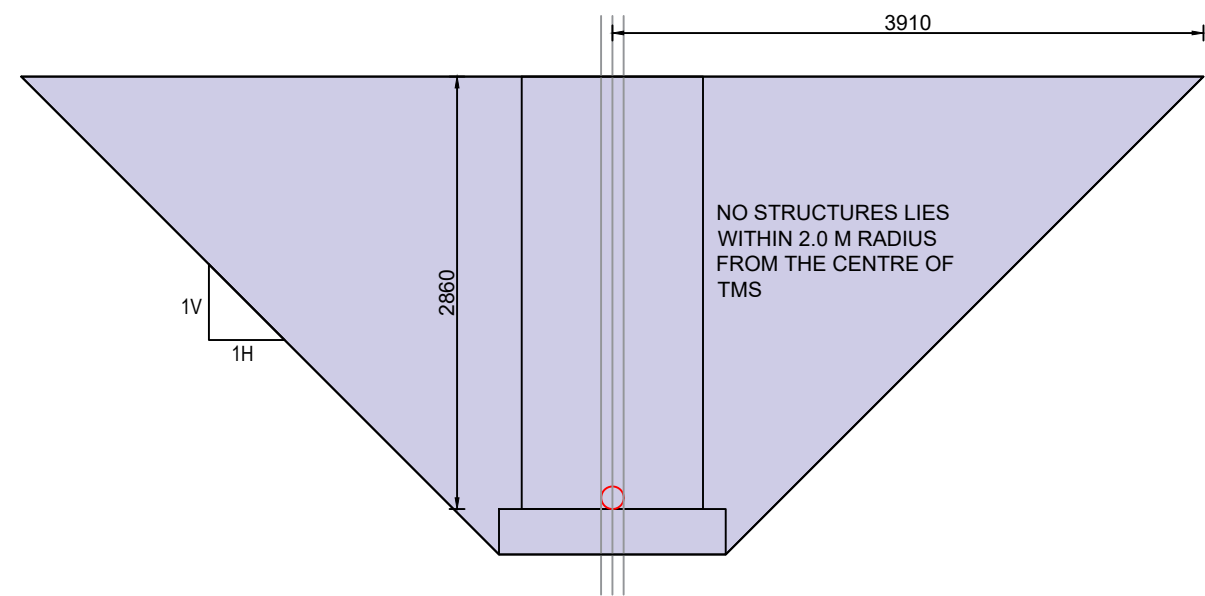
ZOI SECTION DETAIL FOR TMS
