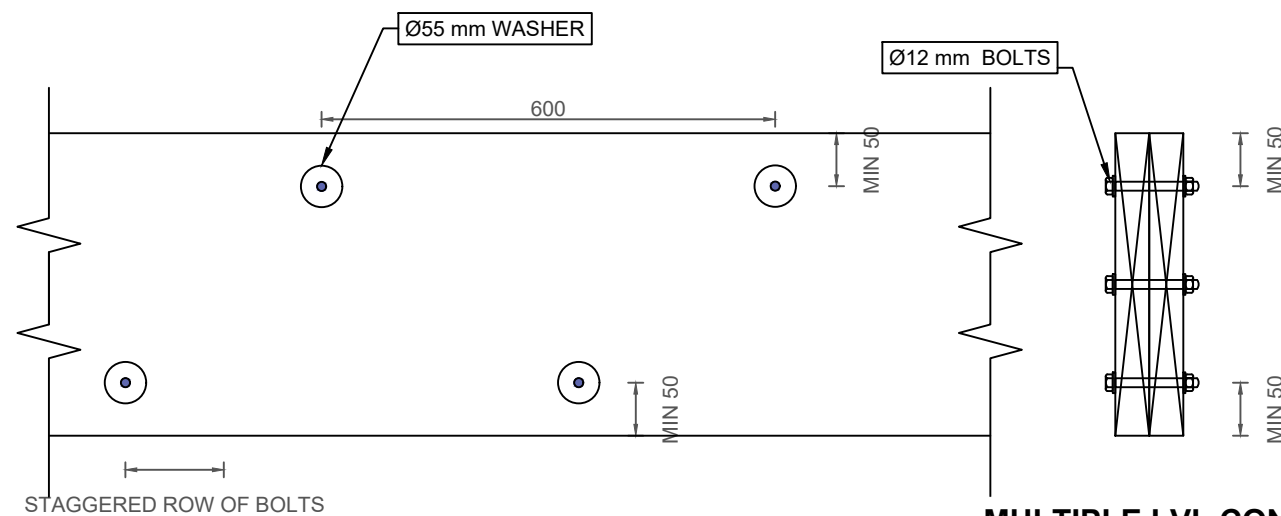
MULTIPLE LVL CONNECTION DETAIL scale 1 : 10
