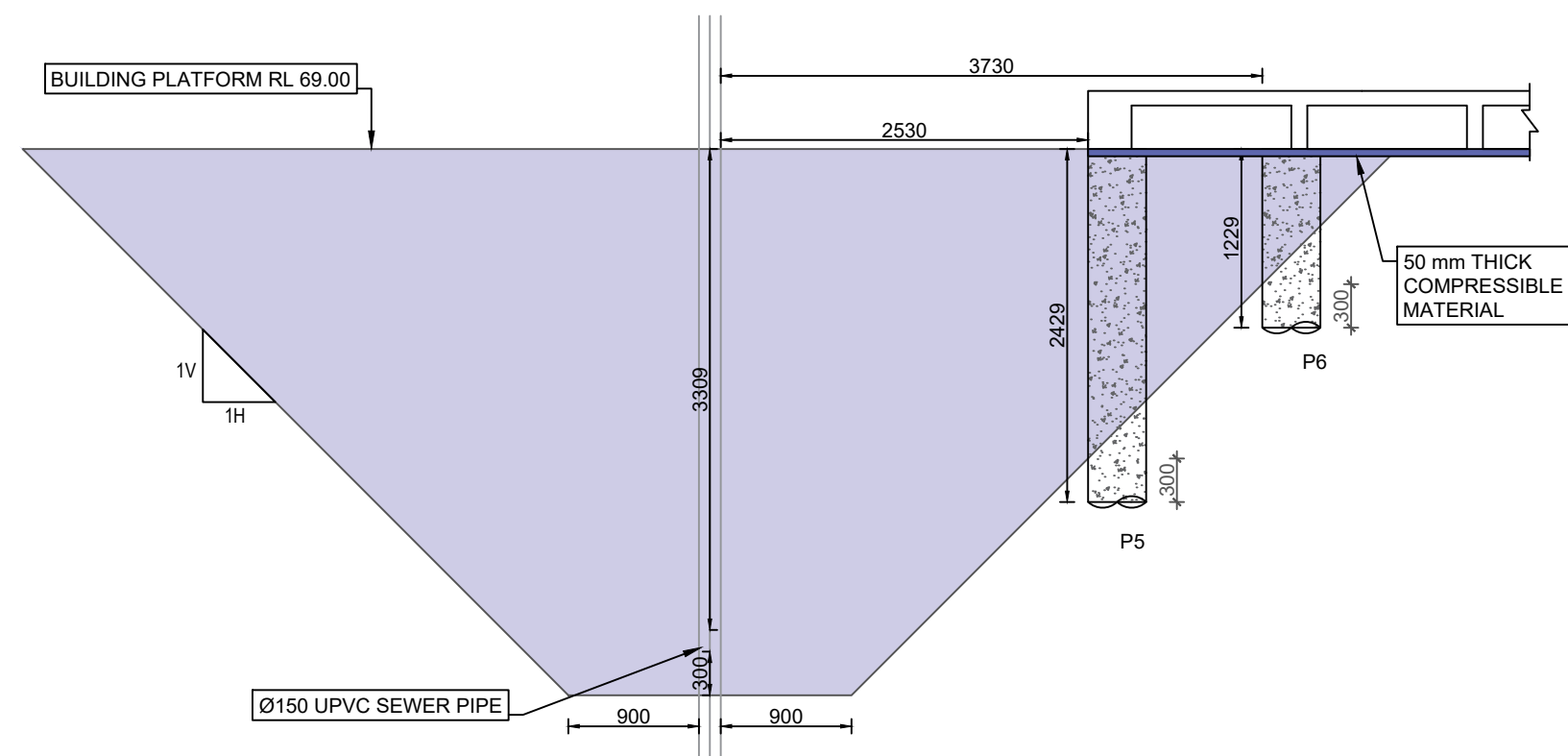
ZOI DETAIL FOR P5 & P6
