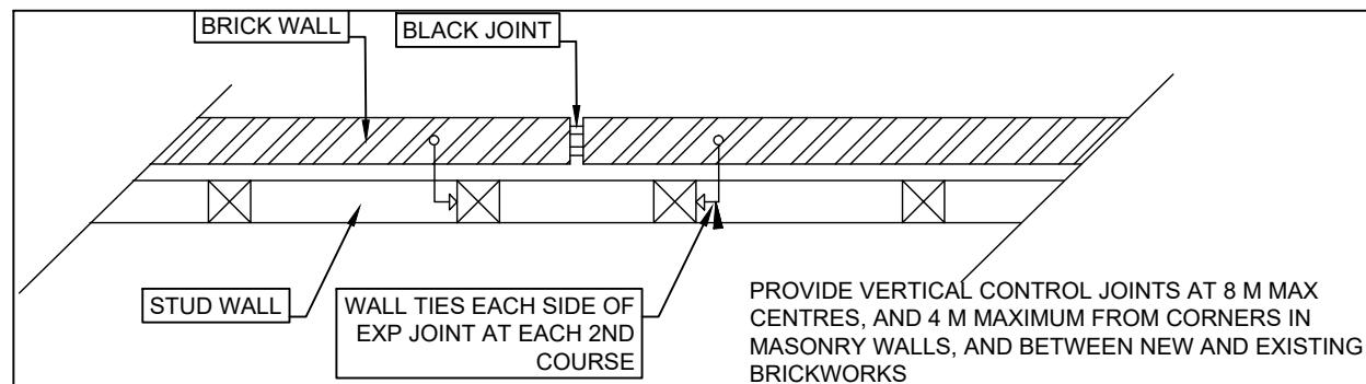
TYPICAL EXPANSION JOINT DETAIL scale 1 : 10
