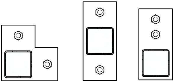
TYPICAL BASE PLATE DETAIL nts
