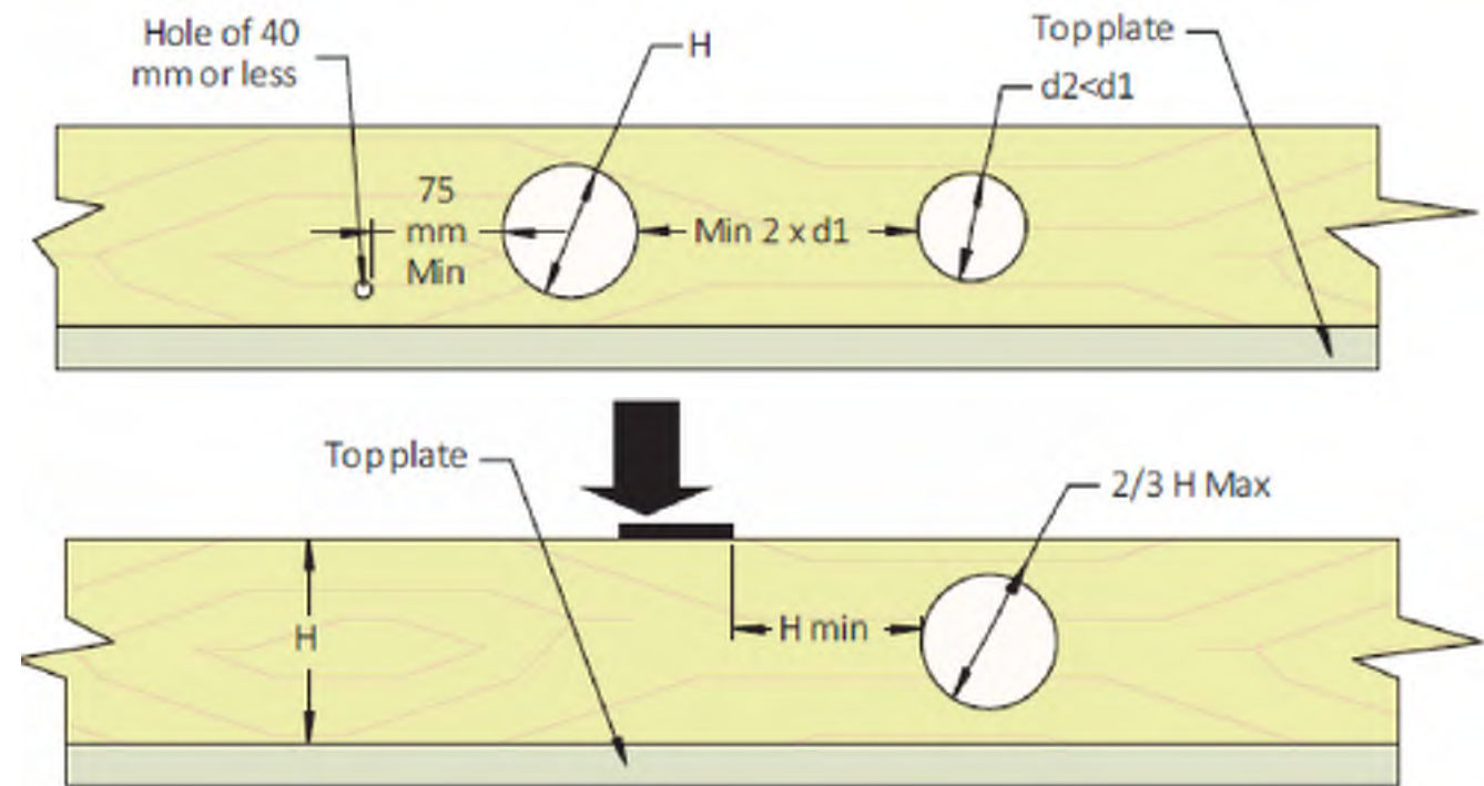
TYPICAL DETAIL OF HOLES IN JOIST nts
