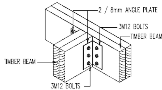
TIMBER BEAM - TIMBER BEAM CONNECTION not to scale
