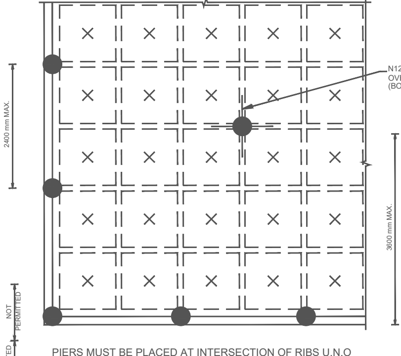
SLAB PIER PLAN VIEW TYP. N.T.S
