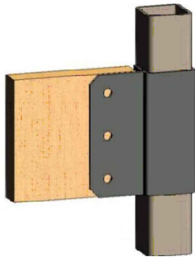
CLEAT FOR SHS-TIMBER BEAM CONNECTION not to scale
