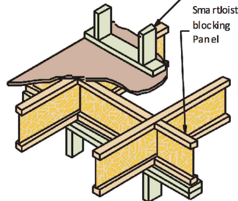
TYPICAL JOIST BLOCKING DETAIL nts
