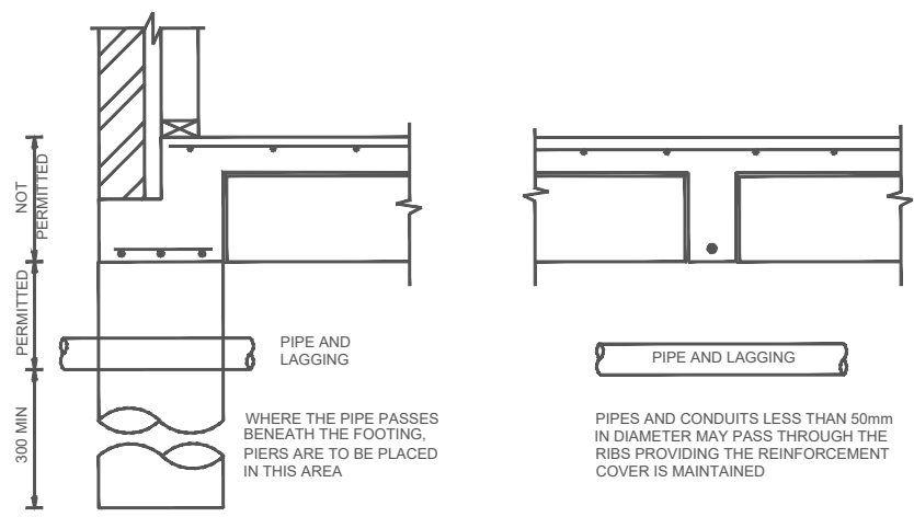
TYPICAL PIPE LAYING UNDER SLAB DETAIL NTS
