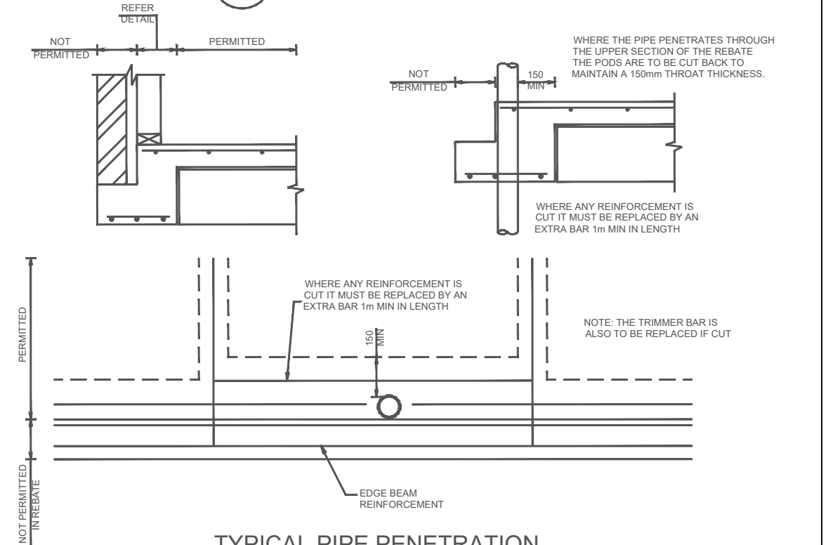
TYPICAL PIPE PENETRATION THROUGH EDGE BEAM DETAIL NTS
