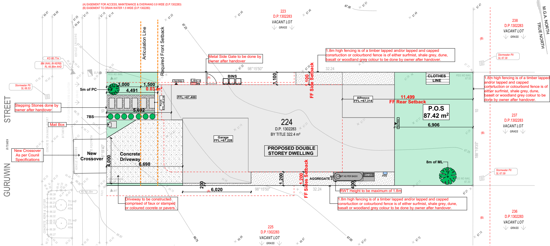
Landscape Plan 1:200
