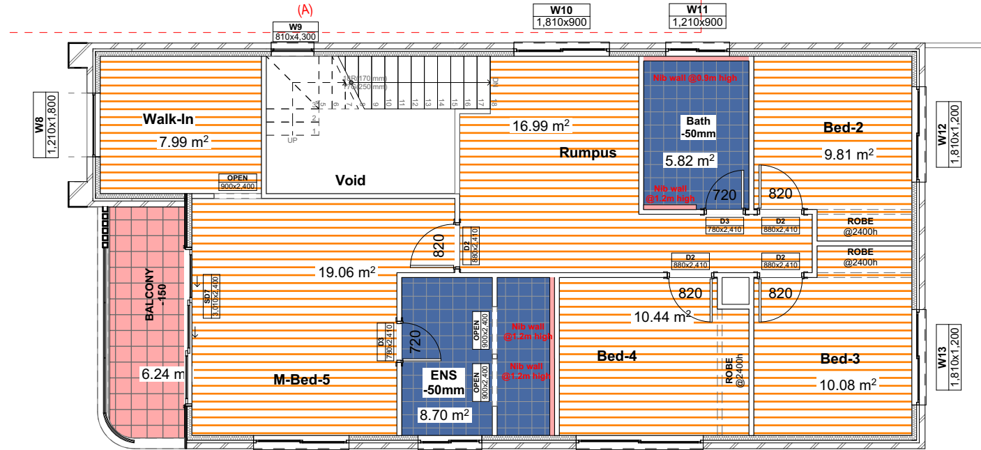
Floor Finish (First Floor) 1:100
