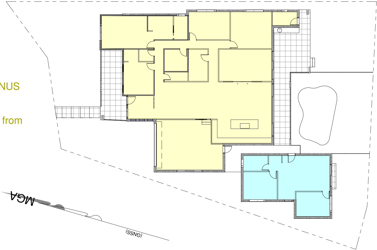
GFA GROUND FLOOR PLAN 1:100
