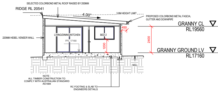
SECTION 2 1:100
