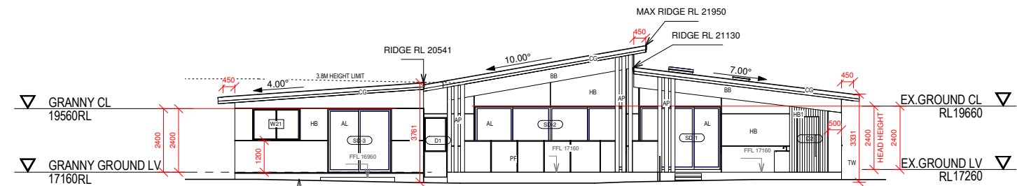
SOUTH ELEVATION 1:100
