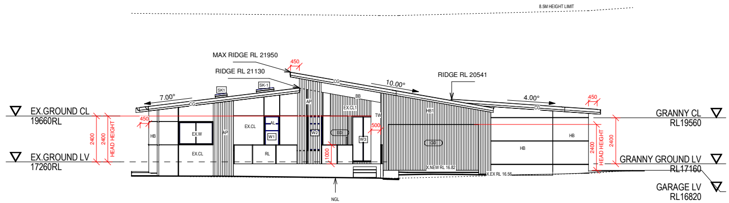
NORTH ELEVATION 1:100
