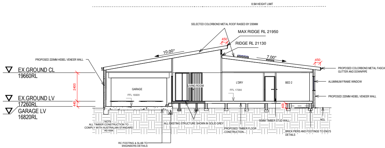
SECTION 1 1:100
