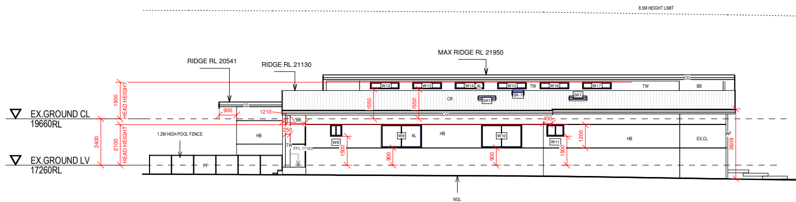
EAST ELEVATION 1:100
