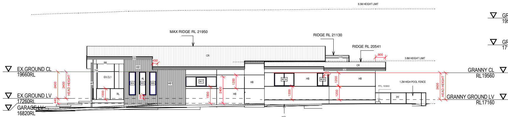
WEST ELEVATION 1:100
