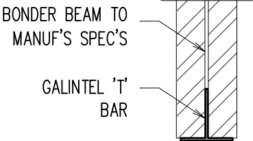
DETAIL – A SCALE 1:20
