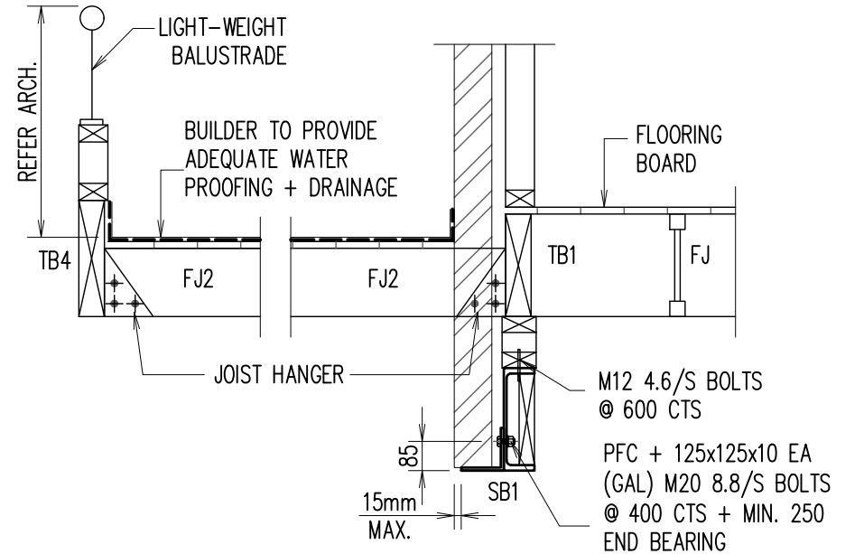
SECTION 4 SCALE 1:20
