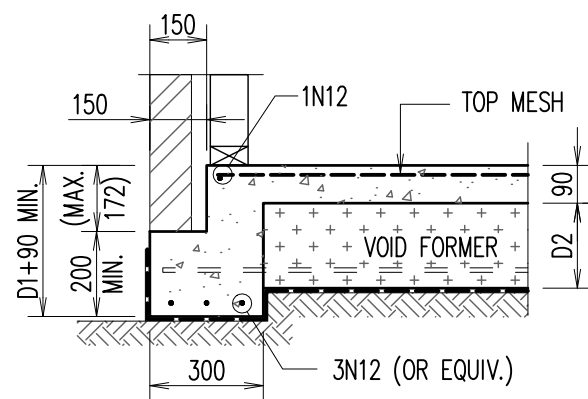
ALTERNATIVELY REFER TO 'IB3 OR DB2' FOR DETAILS
