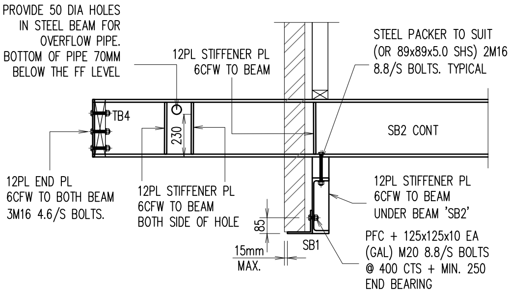
DETAIL – D SCALE 1:20
