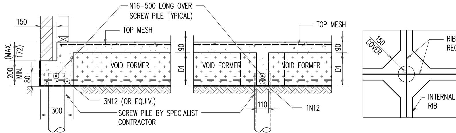
TYPICAL SLAB TO SCREW PILE CONNECTION DETAILS – OPTION 1
