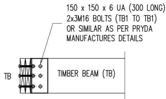
TYPICAL TIMBER BEAM (TB) TO TB DETAIL
