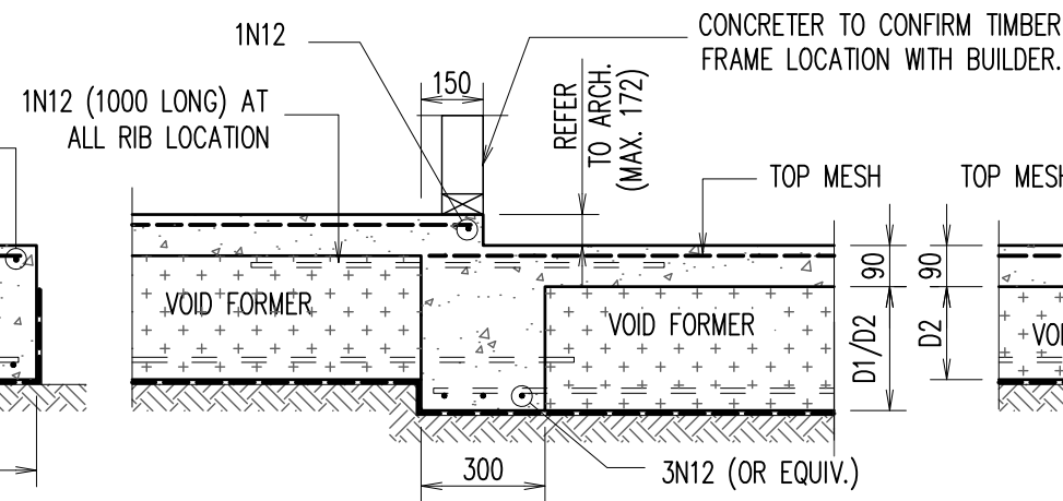
INTERNAL STEPDOWN BEAM – 'IB3' ALTERNATIVELY REFER TO 'DB2' FOR DETAILS
