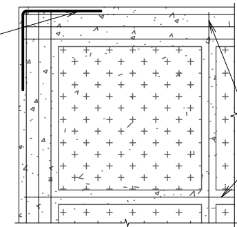
1N12 'L' BARS 600 LEGS TO ALL CORNERS.
