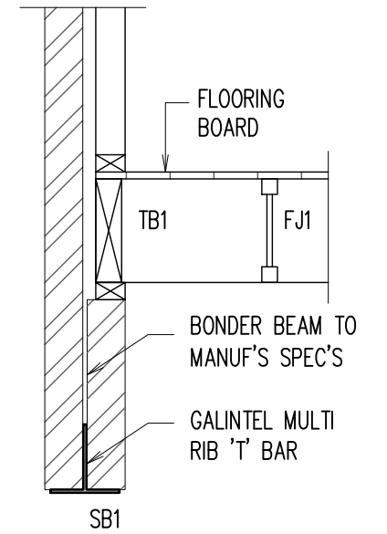
SECTION 4 SCALE 1:20
