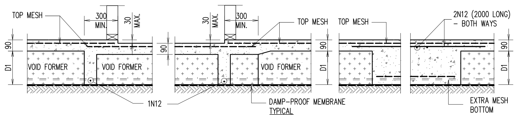
TYPICAL WET AREA STEP DETAIL
