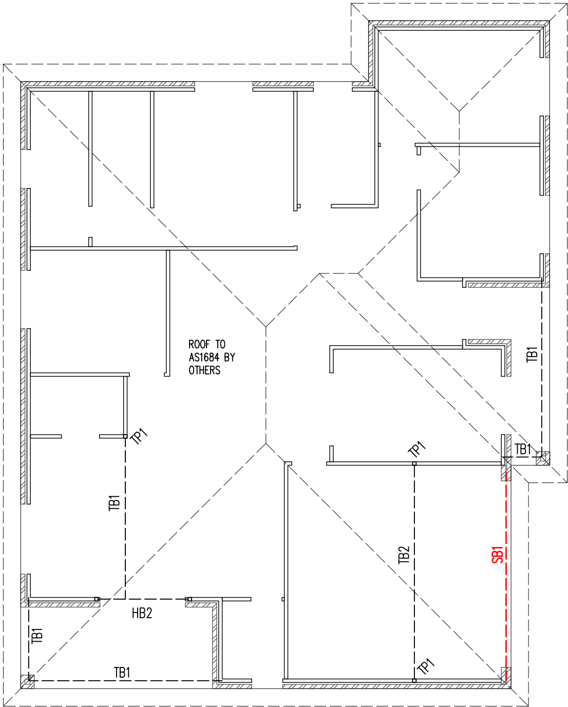
STEEL BEAM AND TIMBER BEAM LAYOUT PLAN
