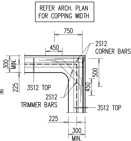
BOND BEAM CORNER DETAIL
