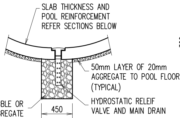
MAIN DRAIN DETAIL
