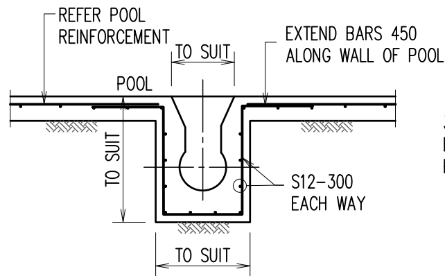
SKIMMER BOX DETAIL
