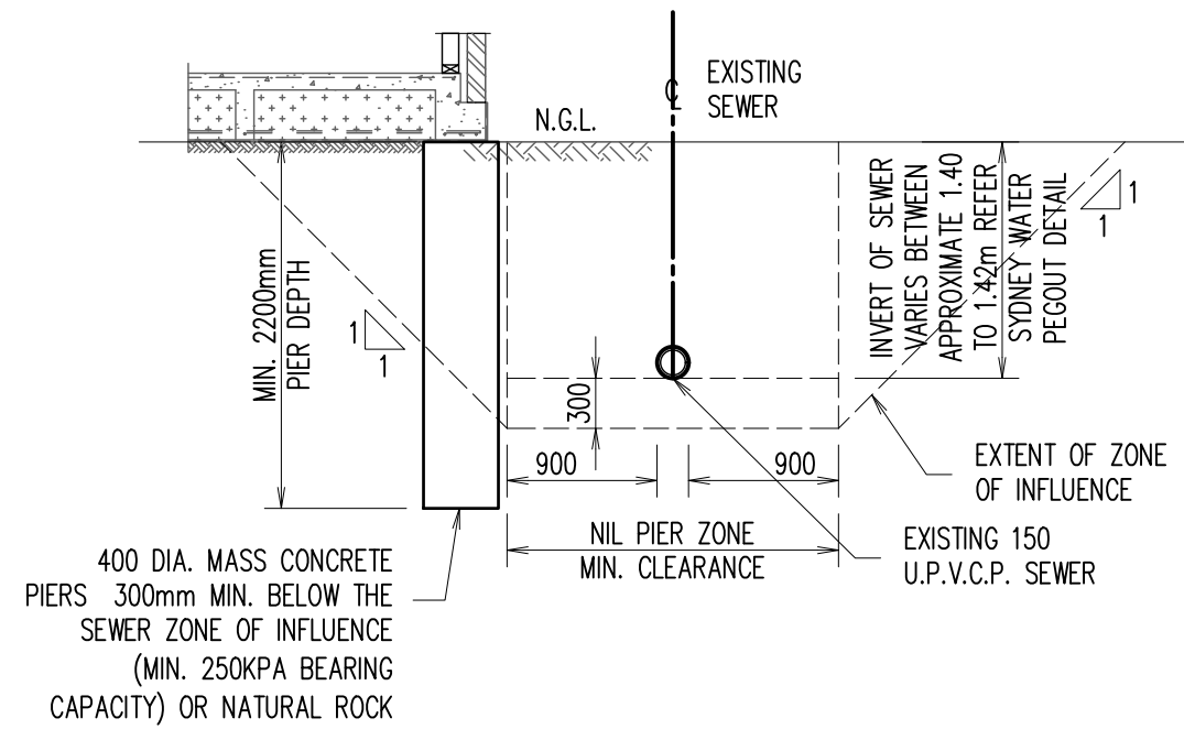
SECTION SCALE 1:50 S1 3
