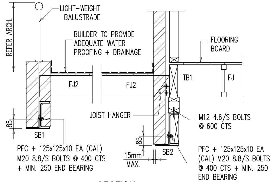
SECTION 5 SCALE 1:20
