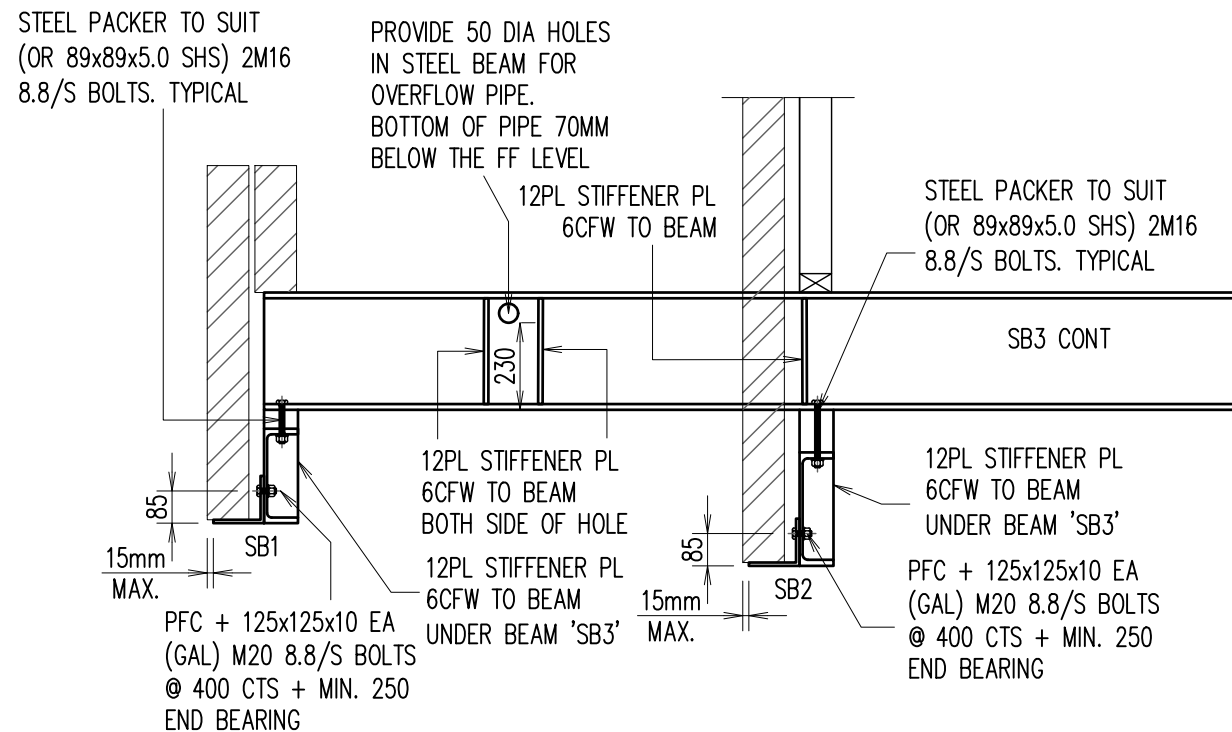
DETAIL - E SCALE 1:20
