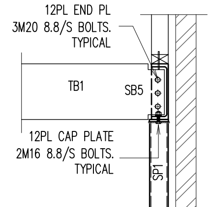
DETAIL - D SCALE 1:20
