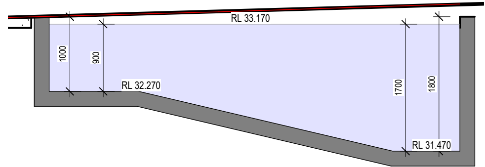
2 POOL LONG SECTION 1 : 50
