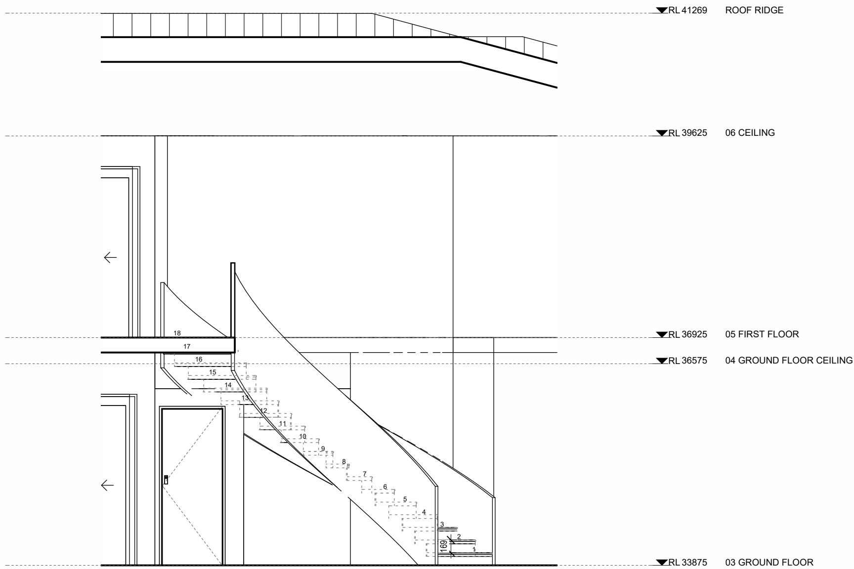
2 GROUND FLOOR STAIR SECTION 1 : 50
