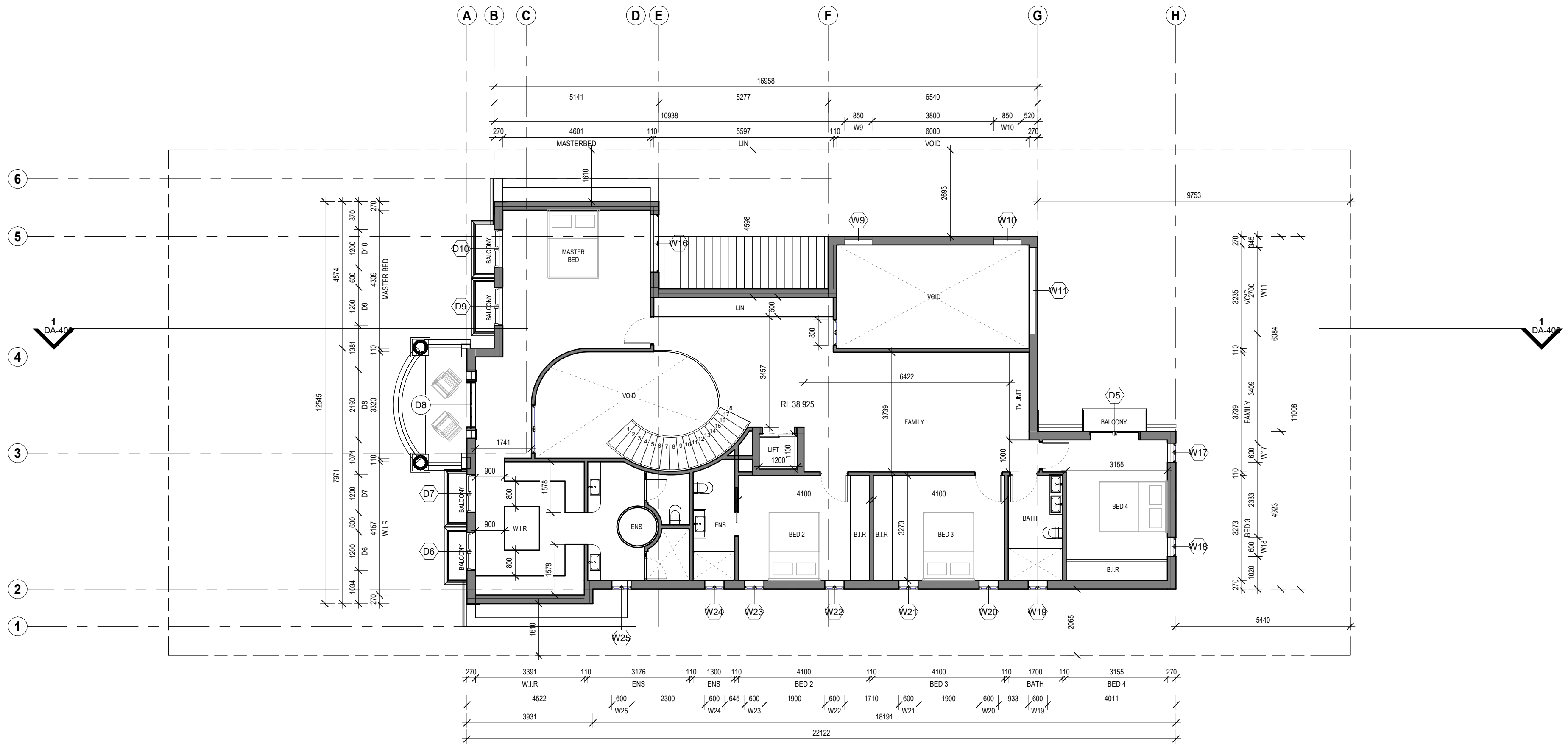
1 05 FIRST FLOOR 1 : 100
