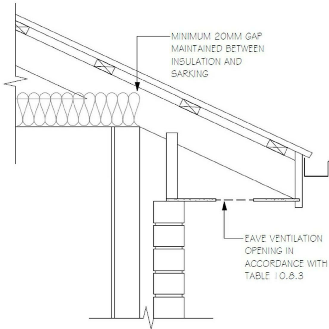
CONDENSATION MANAGEMENT DETAILS
