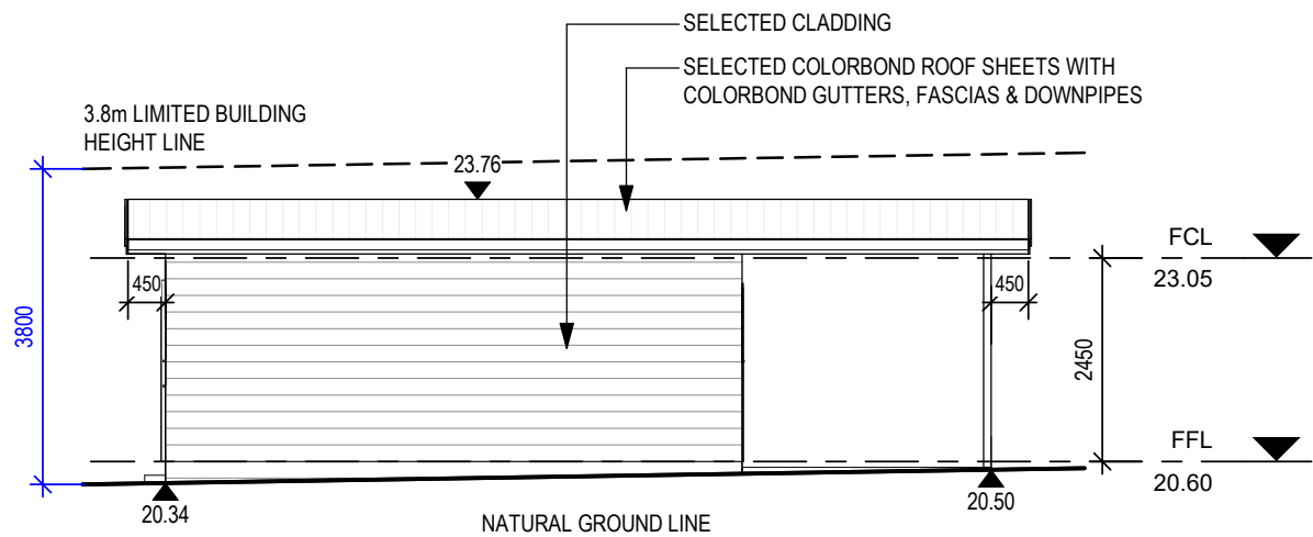
④ NORTH ELEVATION 1 : 100
