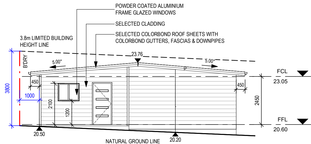
① WEST ELEVATION 1 : 100
