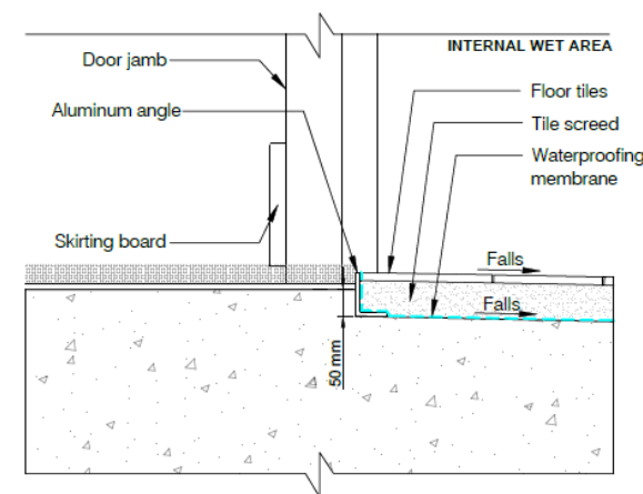
INTERNAL WET AREA DOOR THRESHOLD
