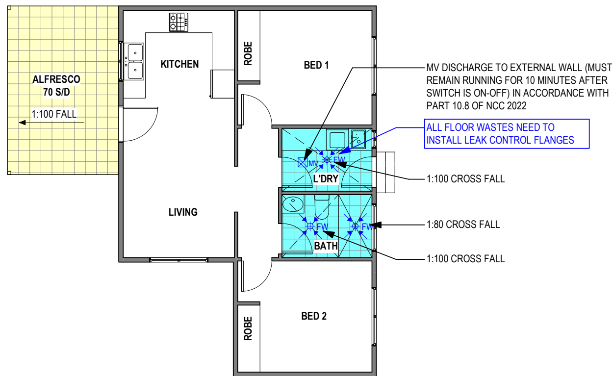
1 PROPOSED GROUND FLOOR PLAN 1 : 100
