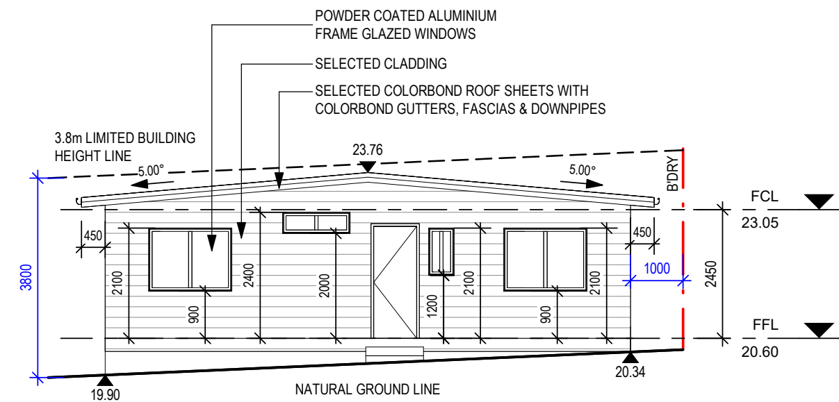
③ EAST ELEVATION 1 : 100
