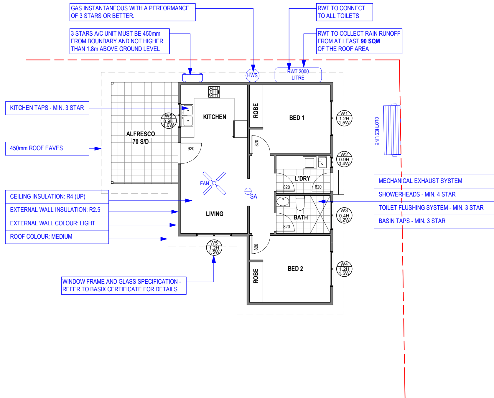
1 PROPOSED GROUND FLOOR PLAN 1 : 100
