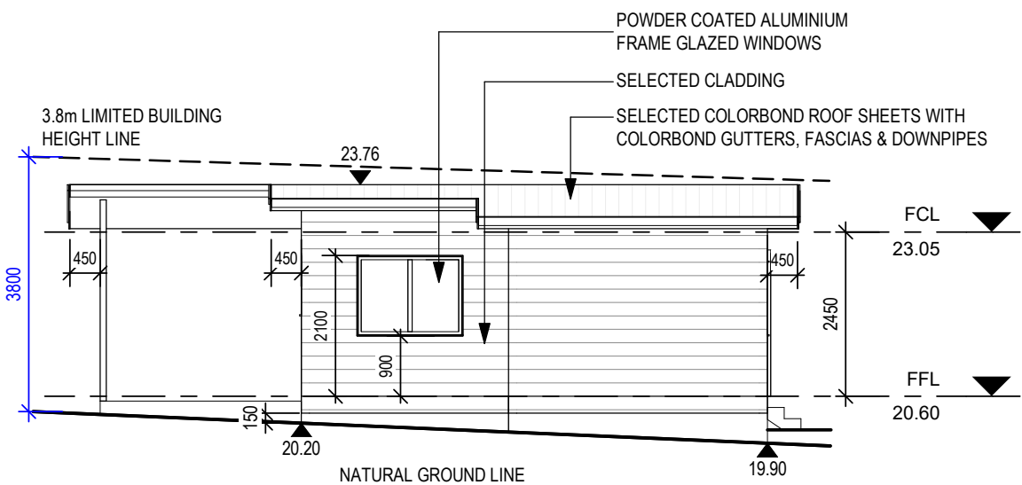
② SOUTH ELEVATION 1 : 100
