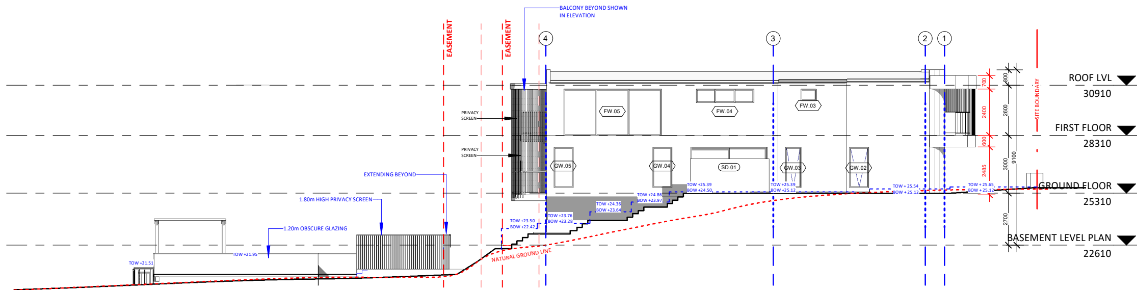
2 SITE ELEVATION - SOUTH WEST ELEVATION 1 : 200
