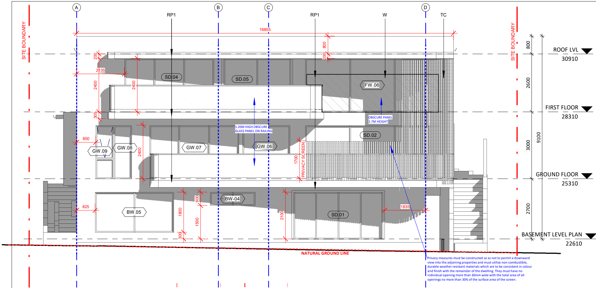
2 SOUTH WEST ELEVATION 1 : 100
