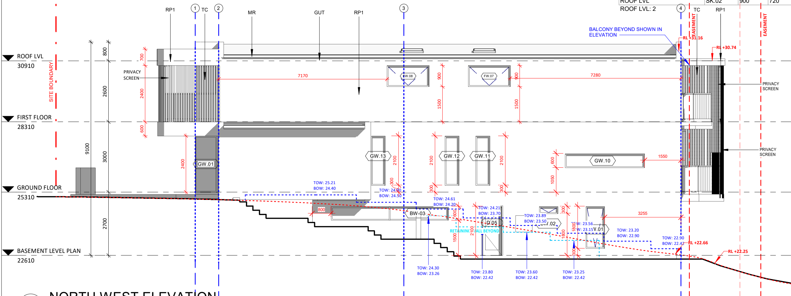
2 NORTH WEST ELEVATION 1 : 100
