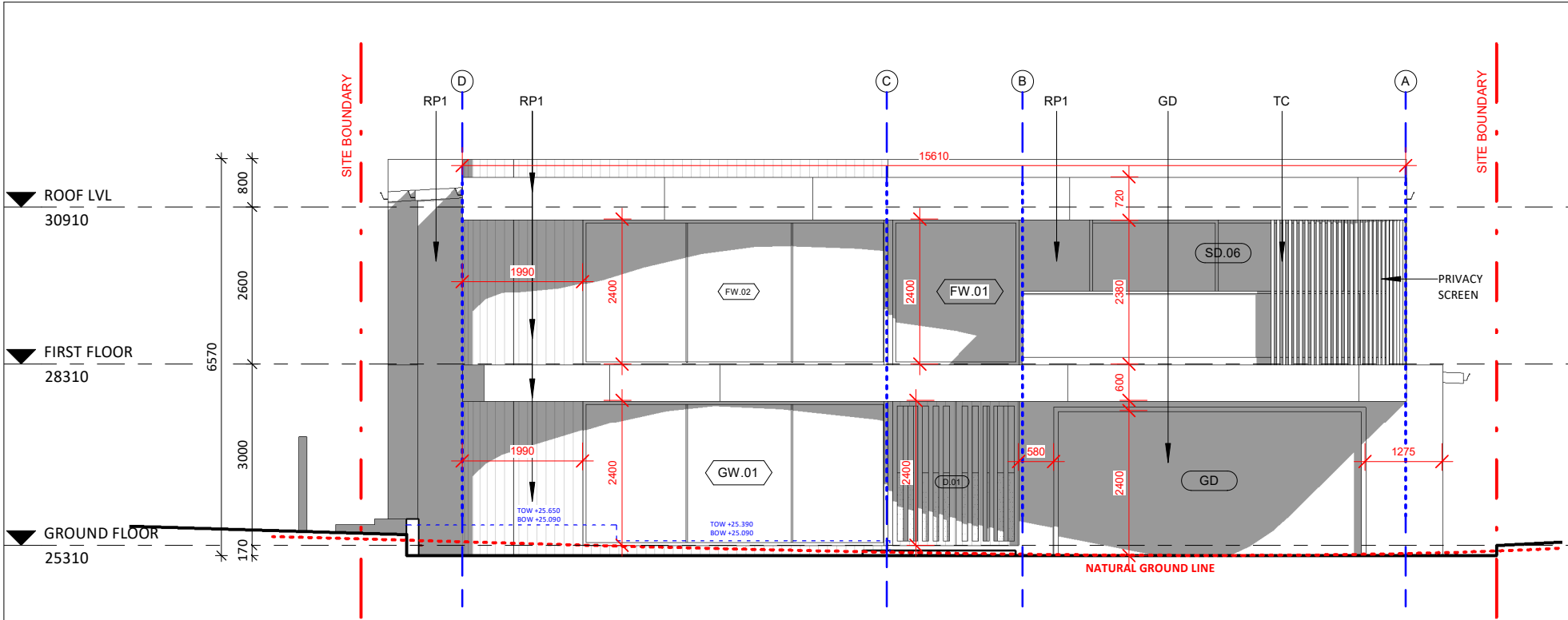
1 NORTH EAST ELEVATION 1 : 100
