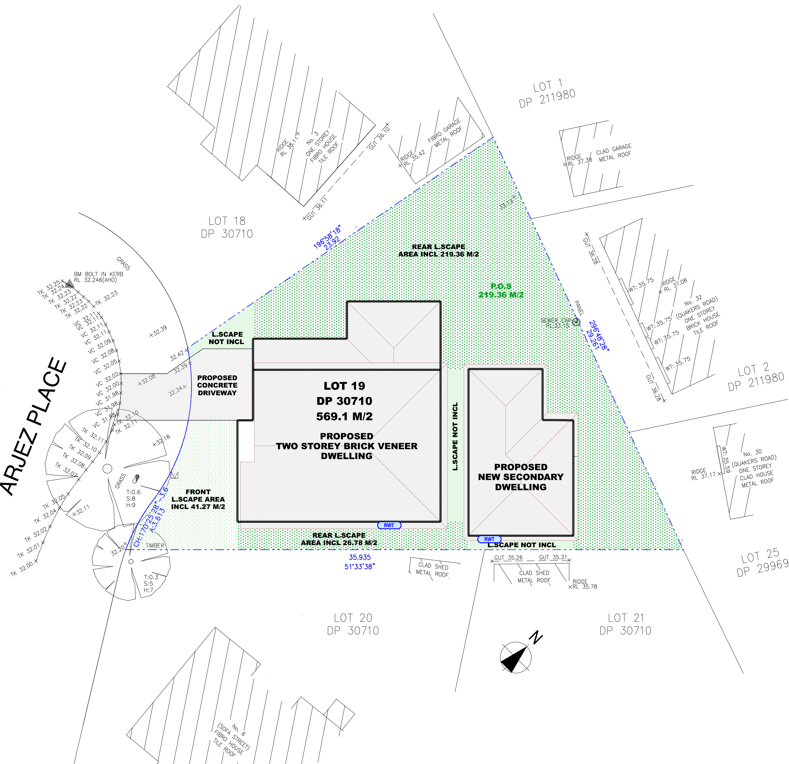
Proposed Landscape Concept Plan 1:150
