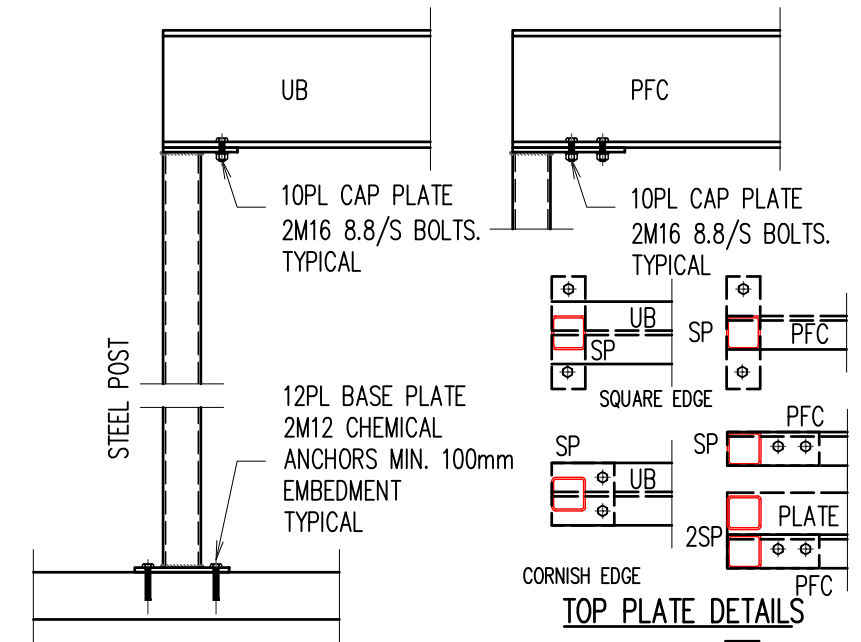
TYPICAL POST TO SLAB DETAIL NOTE: POSTS TO BE SECURELY BRACED TO STUD FRAMEWORK
