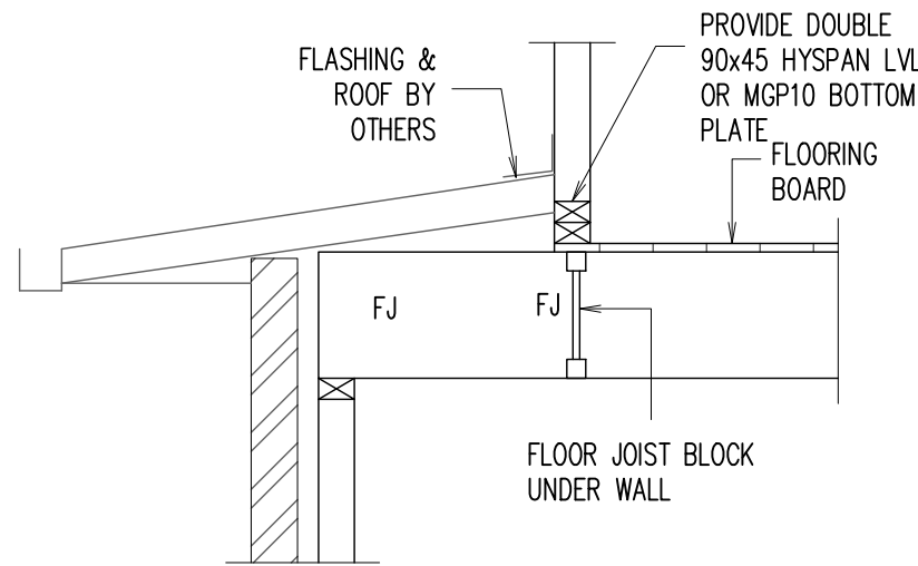
SECTION 4 SCALE 1:20
