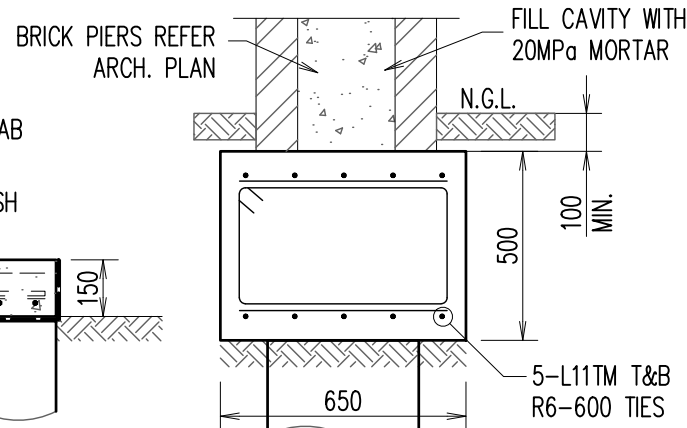
STRIP FOOTING (SF1) DETAILS
