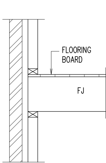
SECTION 1 SCALE 1:20
