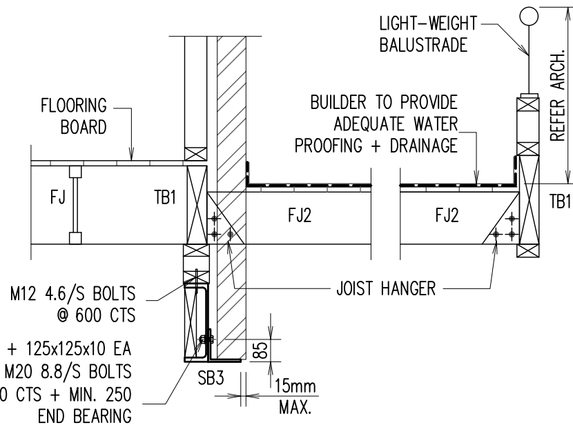
SECTION 7 SCALE 1:20
