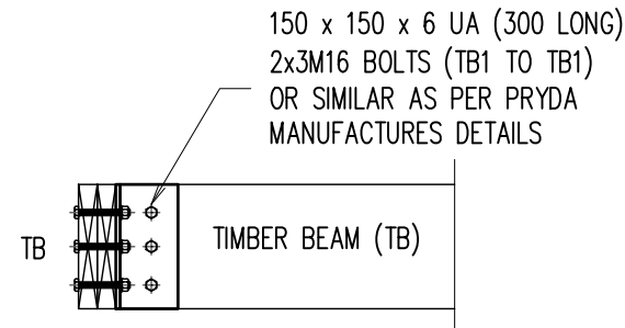
TYPICAL TIMBER BEAM (TB) TO TB DETAIL
