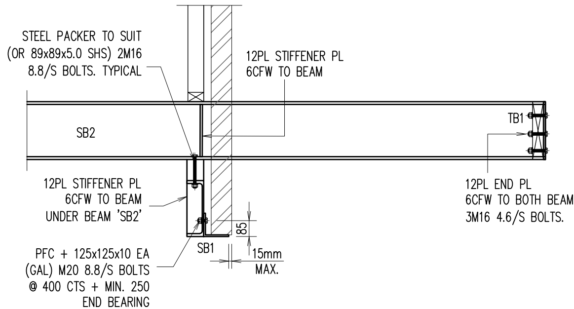
DETAIL - D SCALE 1:20
