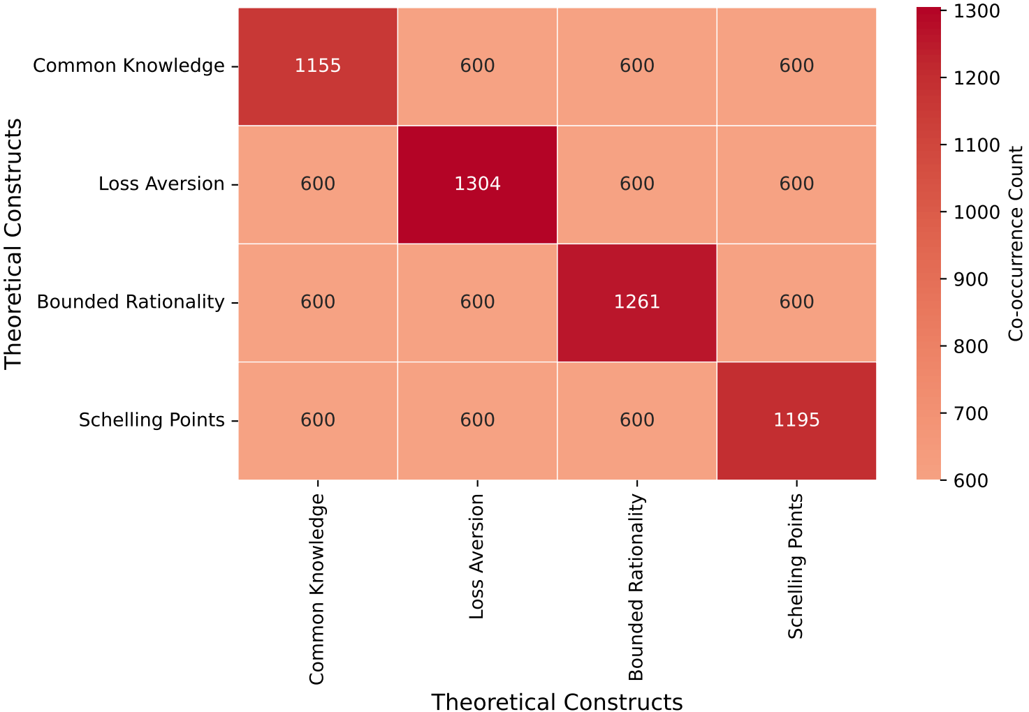
Co-occurrence Matrix of Theoretical Constructs
