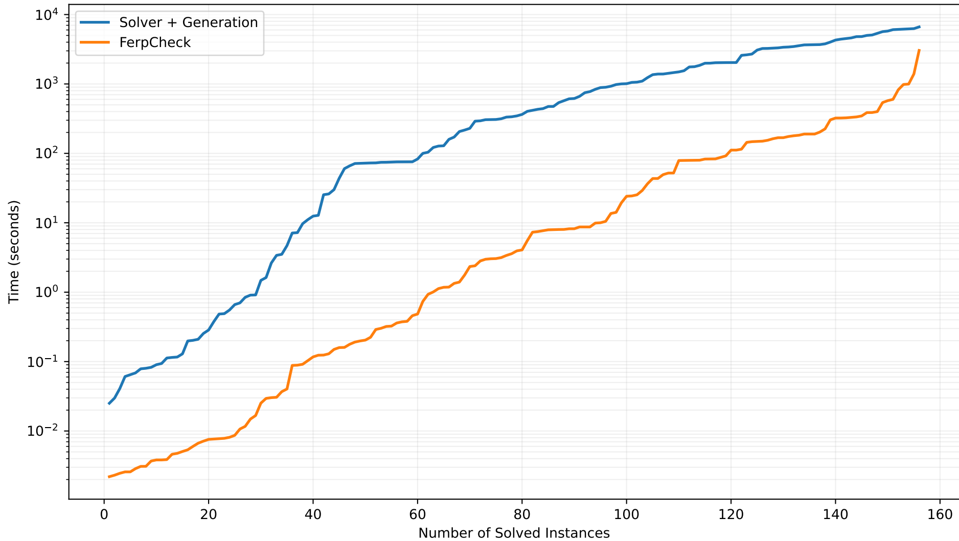
Cactus Plot: Solving vs Checking
