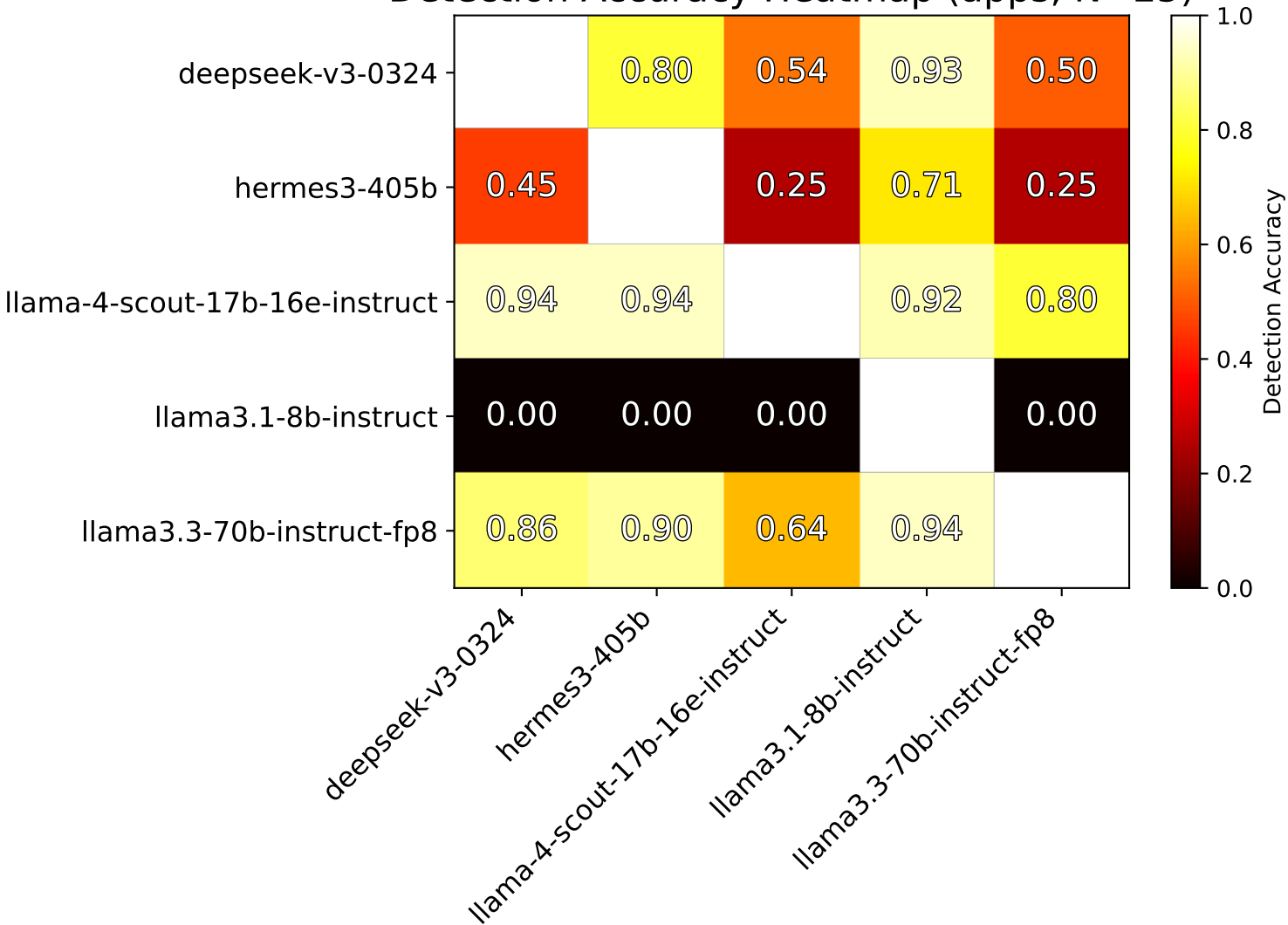
Detection Accuracy Heatmap (apps, N=25)
