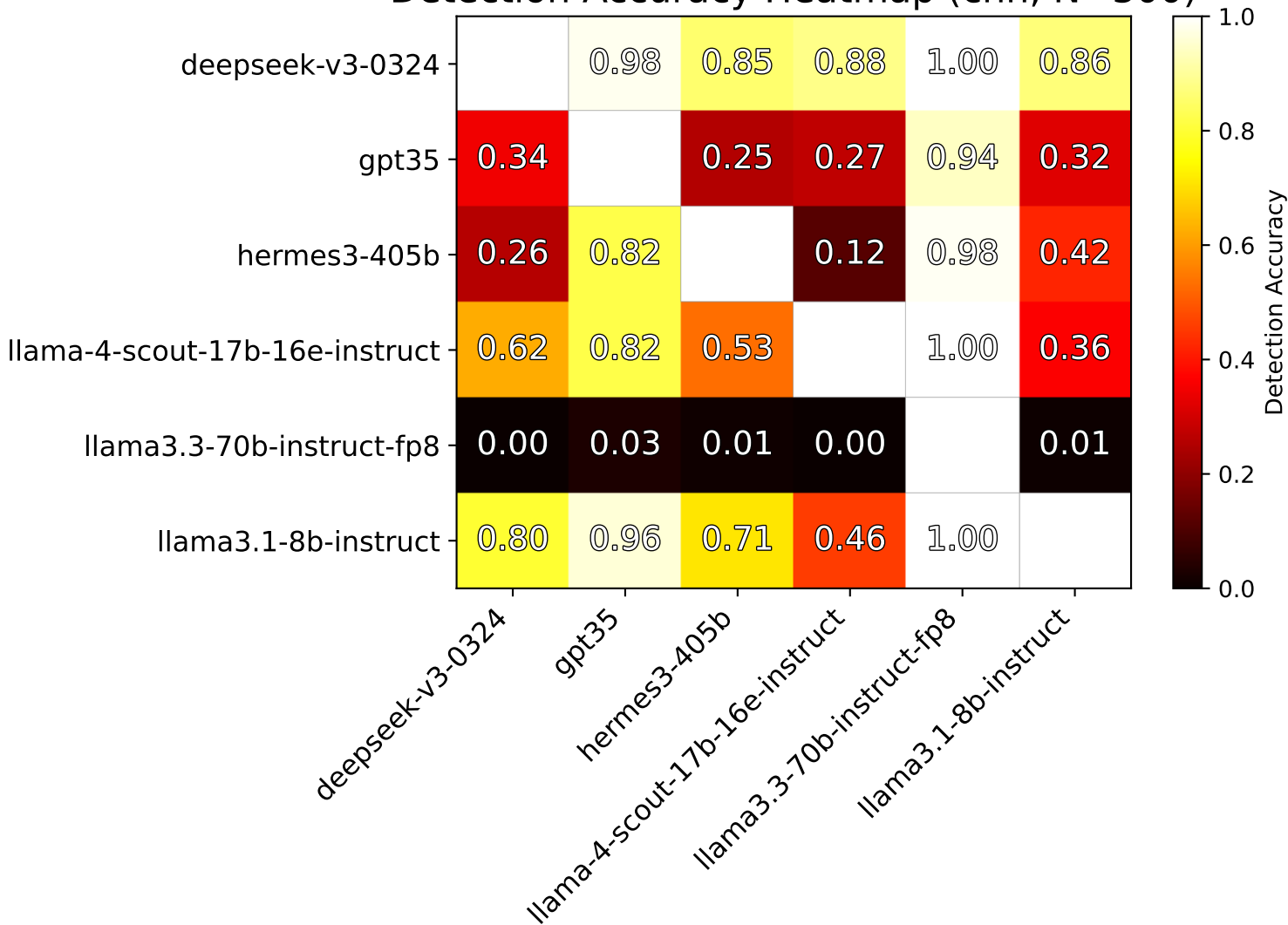
Detection Accuracy Heatmap (cnn, N=300)
