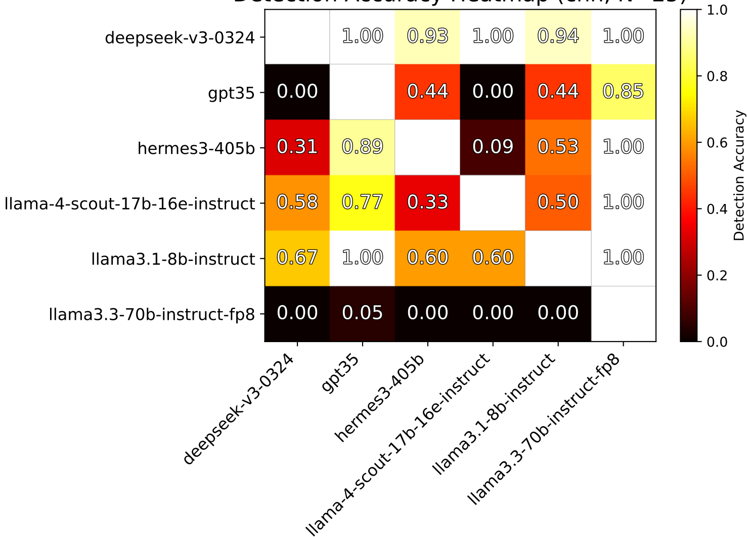
Detection Accuracy Heatmap (cnn, N=25)
