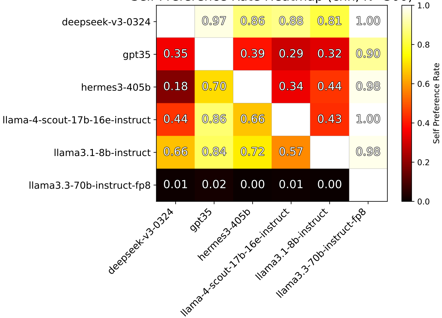
Self Preference Rate Heatmap (cnn, N=300)
