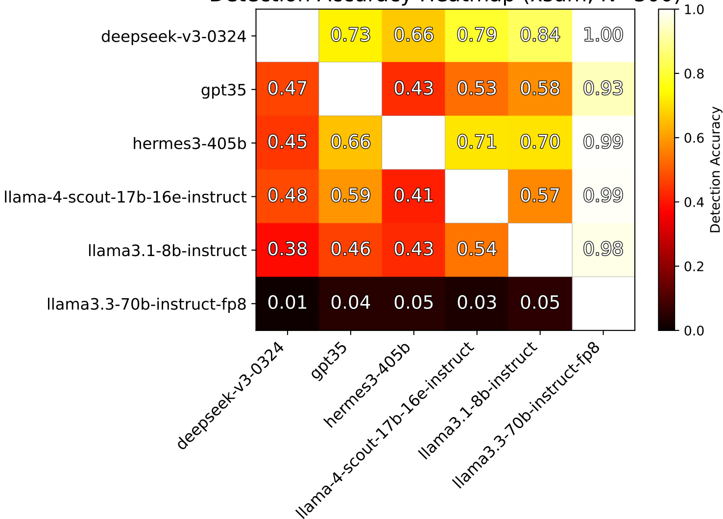
Detection Accuracy Heatmap (xsum, N=300)
