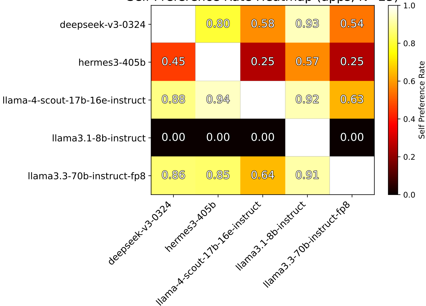
Self Preference Rate Heatmap (apps, N=25)
