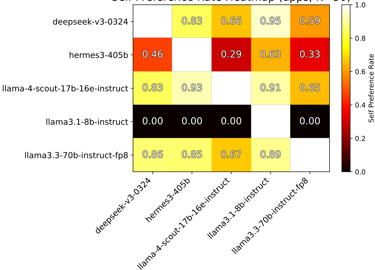
Self Preference Rate Heatmap (apps, N=30)
