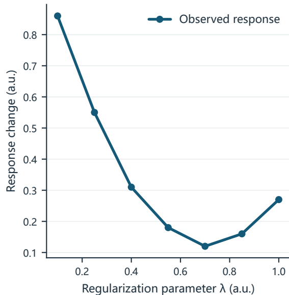
One-parameter effect
