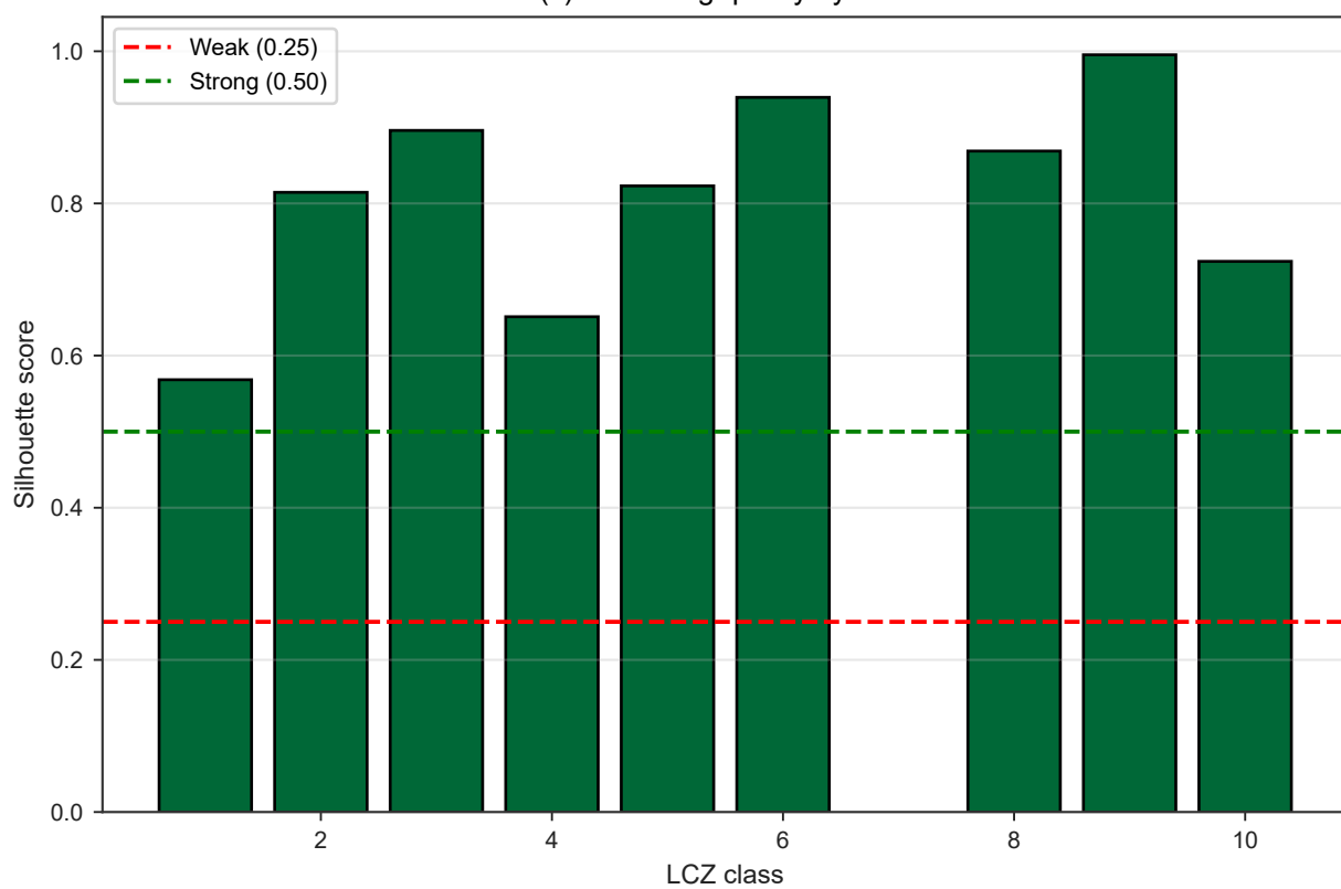
(c) Clustering quality by LCZ
