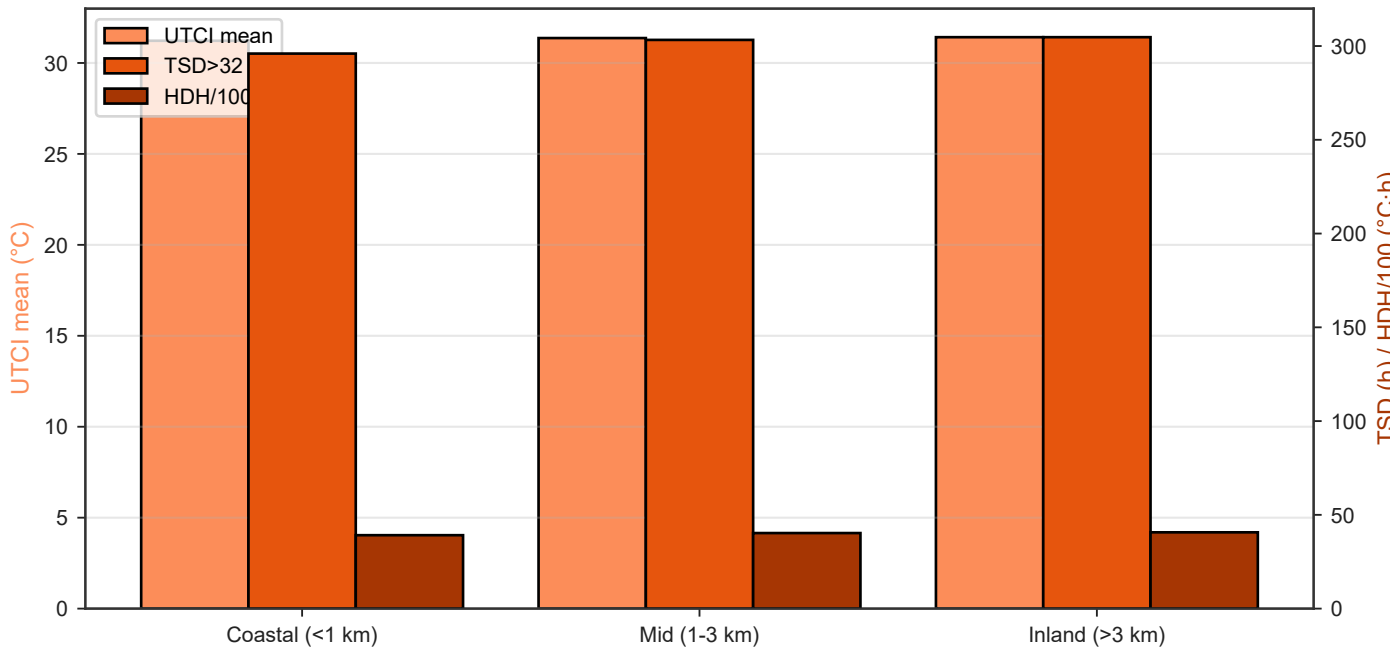
(e) Coastal vs inland exposure ladder
