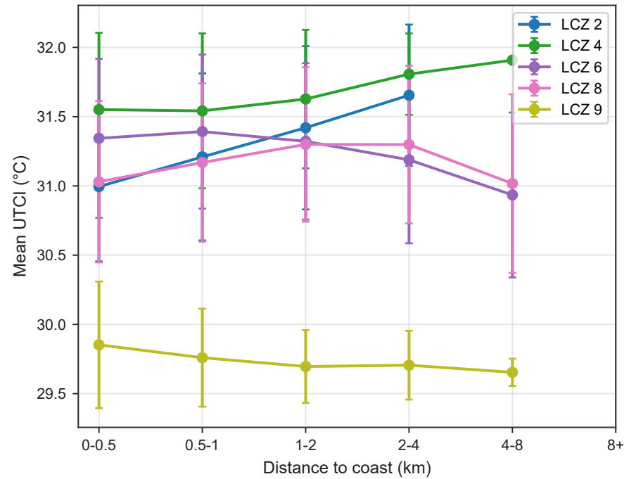
(a) UTCI gradient by coast distance
