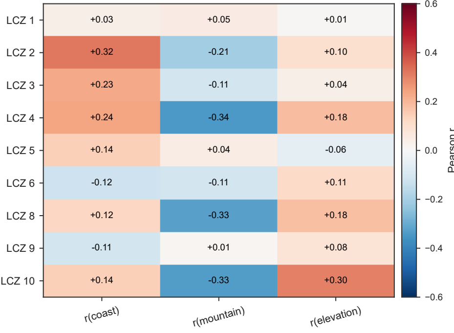
(c) Within-LCZ Pearson r (UTCI ~ distance)
