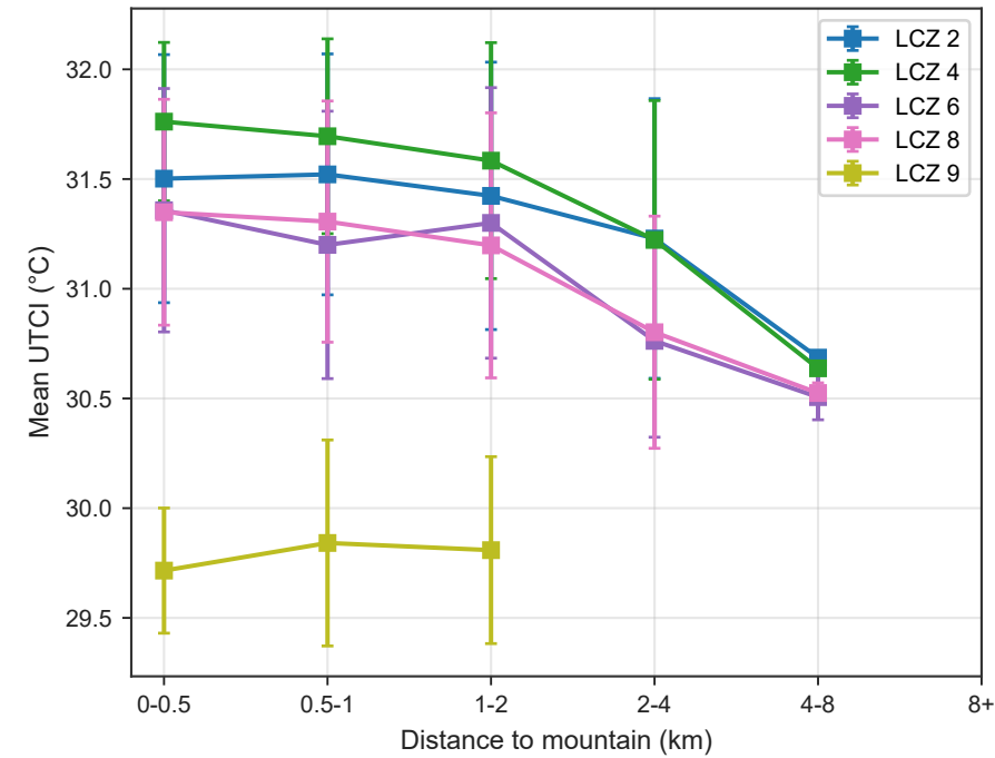
(b) UTCI gradient by mountain distance
