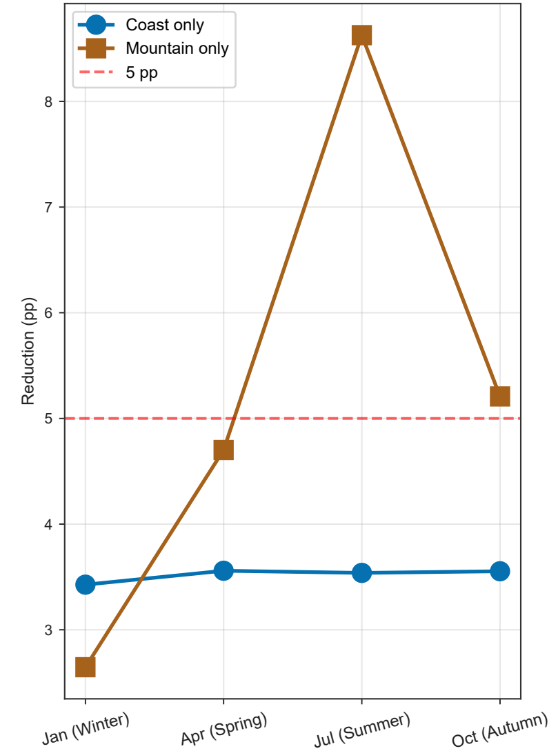
(c) Mechanism stability across seasons
