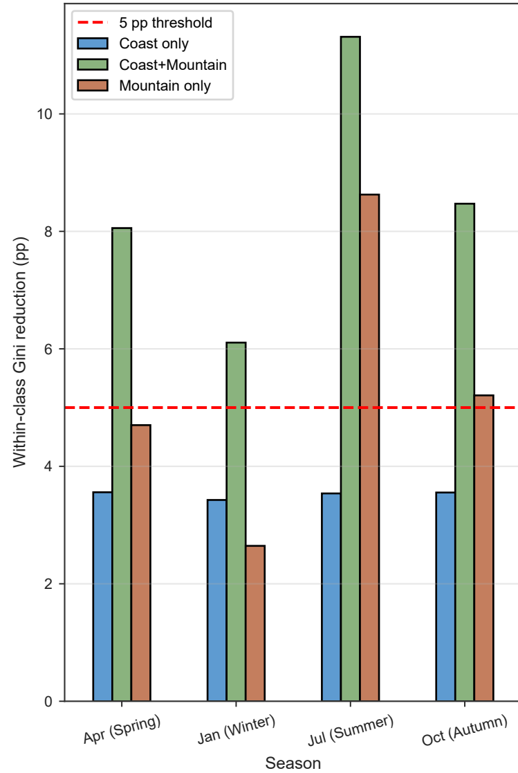
(a) Gini reduction by season
