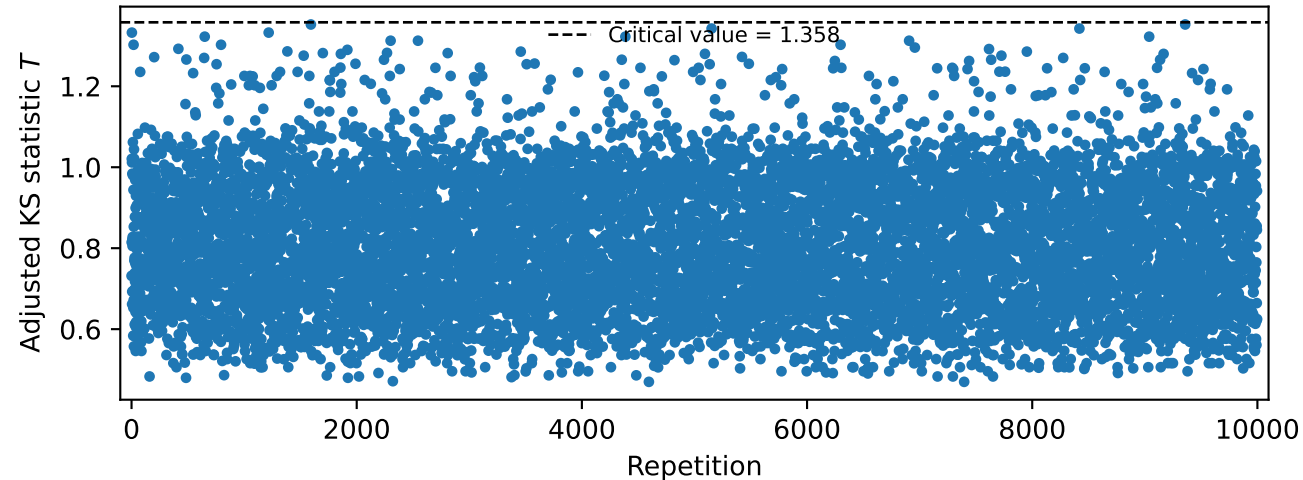
Smirnov test across 10.000 repetitions
