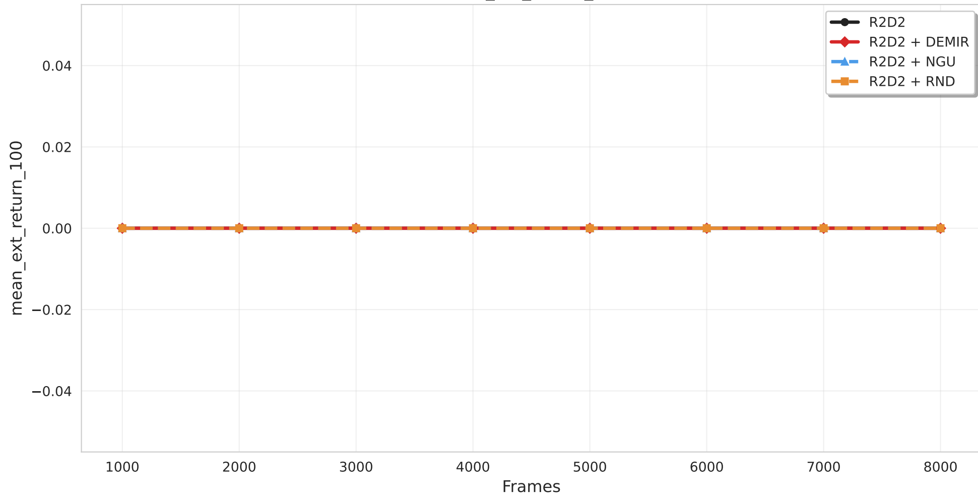
mean_ext_return_100
