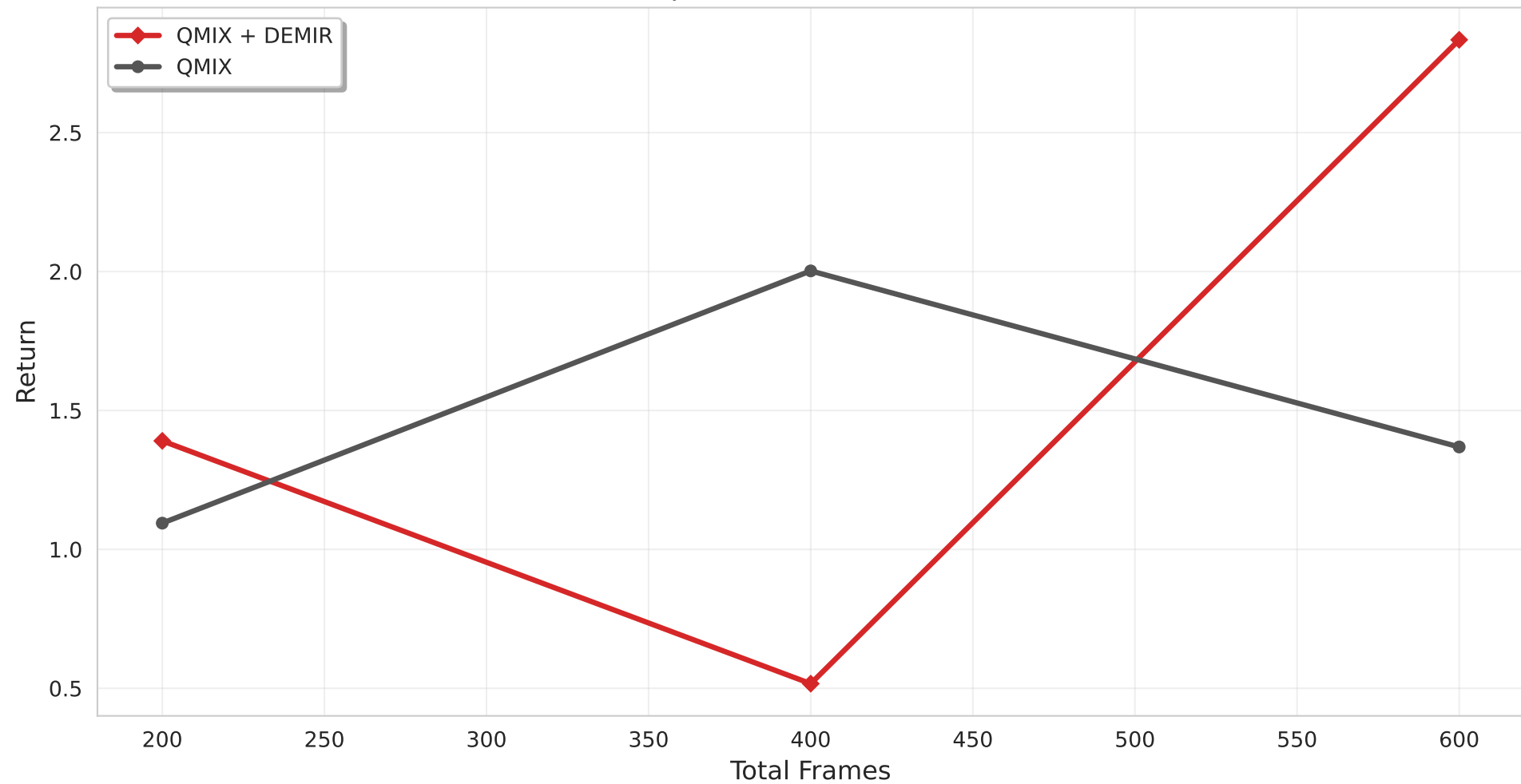
Episode Return (Mean)
