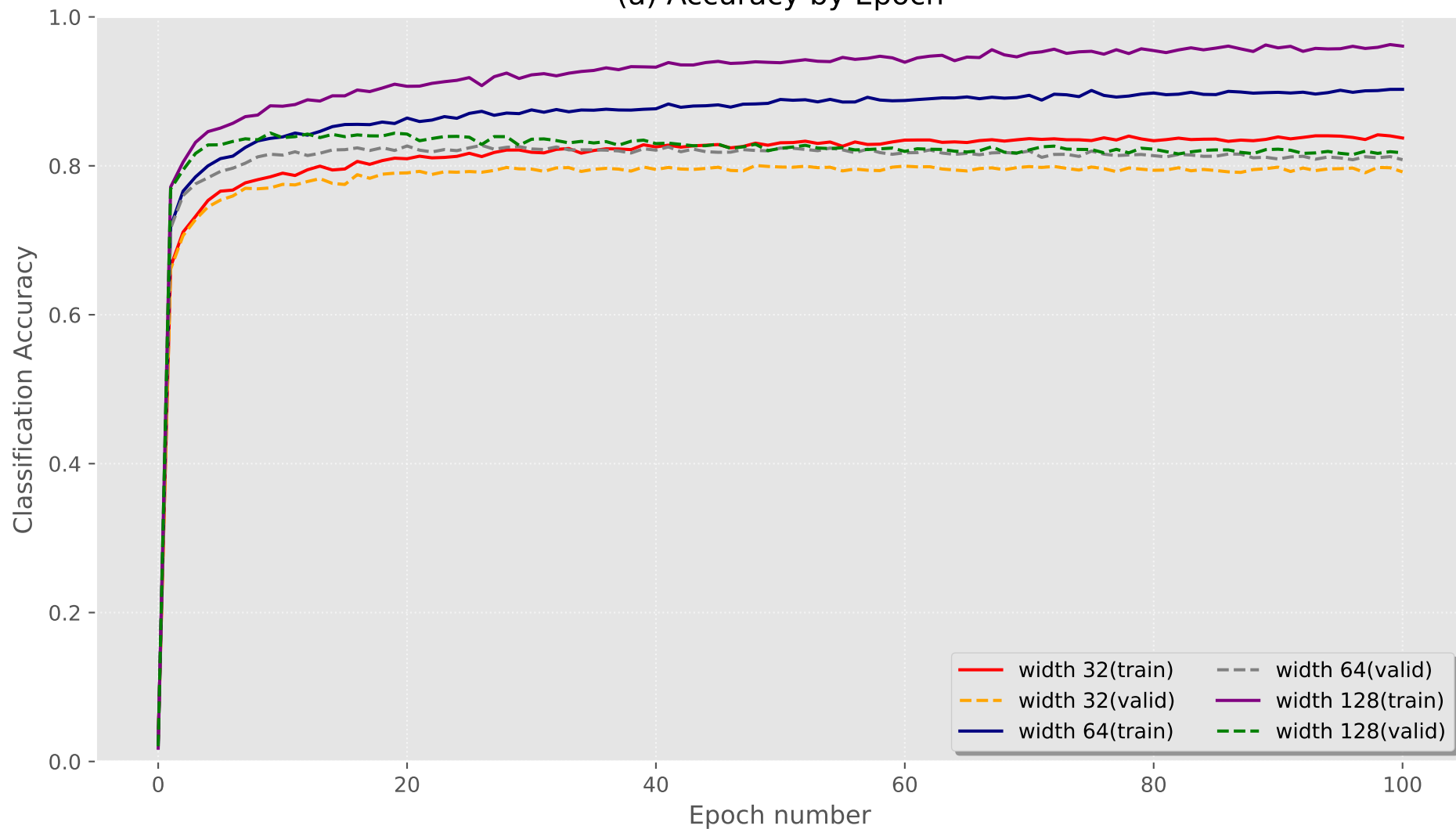
(a) Accuracy by Epoch
