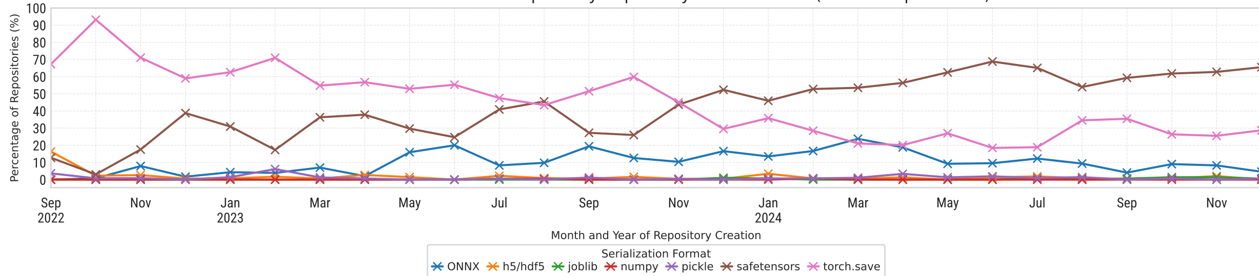
Serialization Formats Adoption by Repository Creation Date (Recent Repositories)
