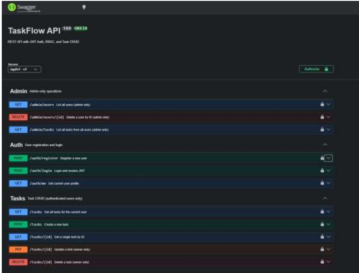
Figure 1: Swagger UI at /api/v1/docs showing all 11 API endpoints across Admin, Auth, and Tasks groups
