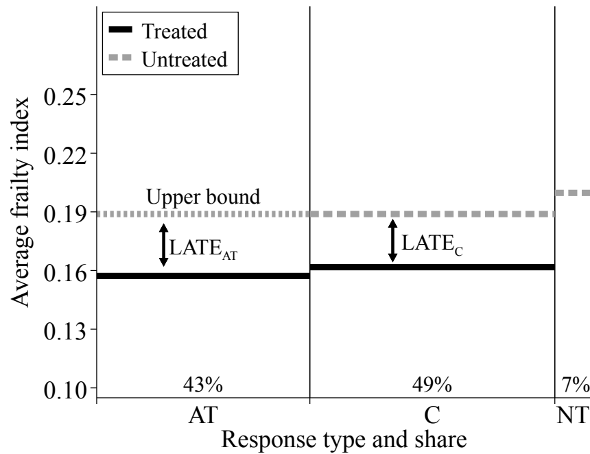
FIGURE B.2 – Treated and untreated potential outcomes by type
