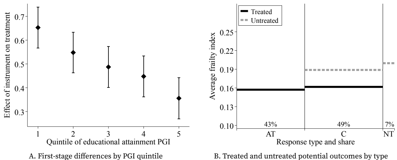
FIGURE 4 – Evidence on differences in the first-stage and second-stage potential outcomes
