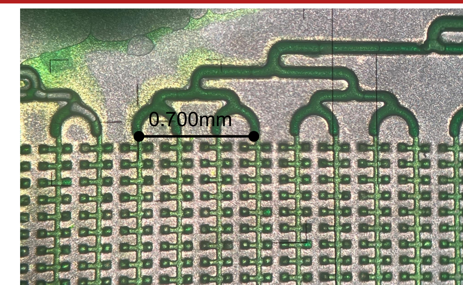
Figure 4: Microscope image of the fully bonded microfluidic device testing with green dye
