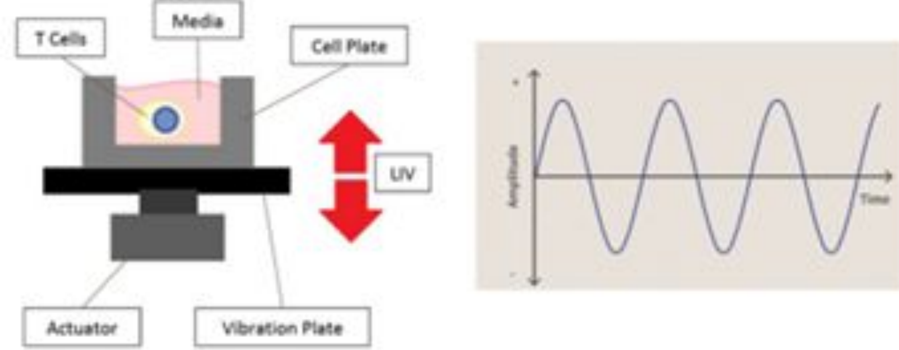
Fig 1. Typical LIV experimental setup and signal parameters. 4
