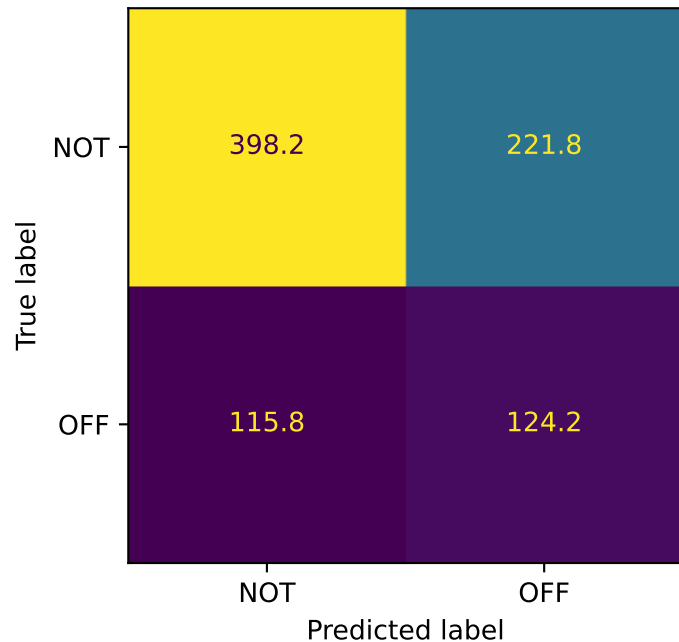
CNN — Cross-domain: HASOC → OLID (mean over 5 seeds)
