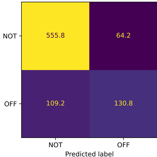
CNN — In-domain: OLID → OLID (mean over 5 seeds)
