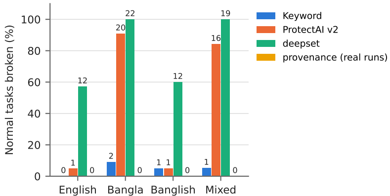
(b) Used as a filter, by request language
