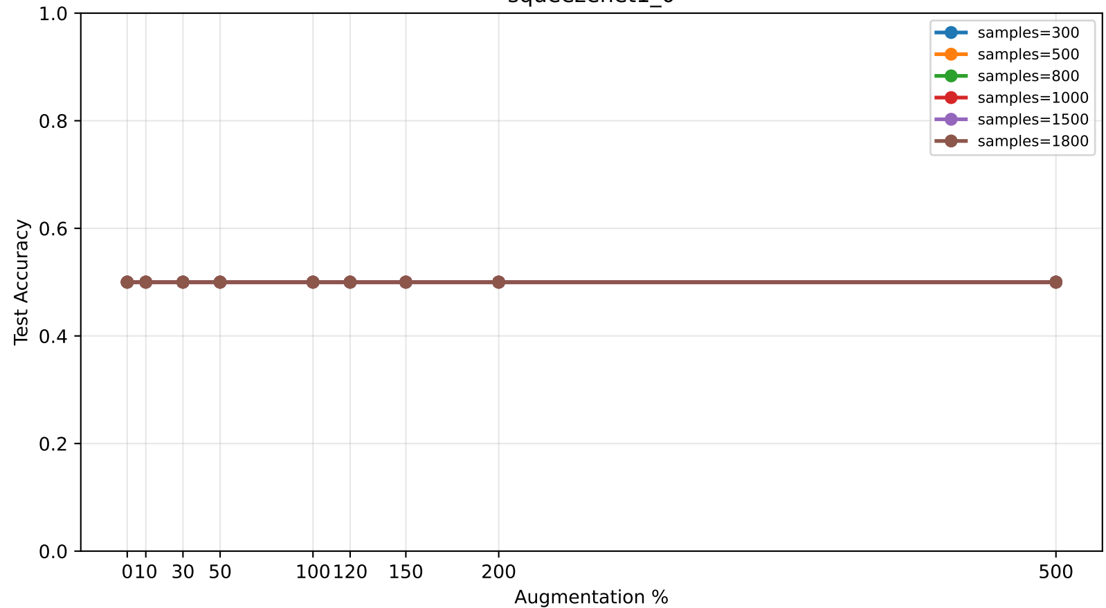
squeezenet1_0
