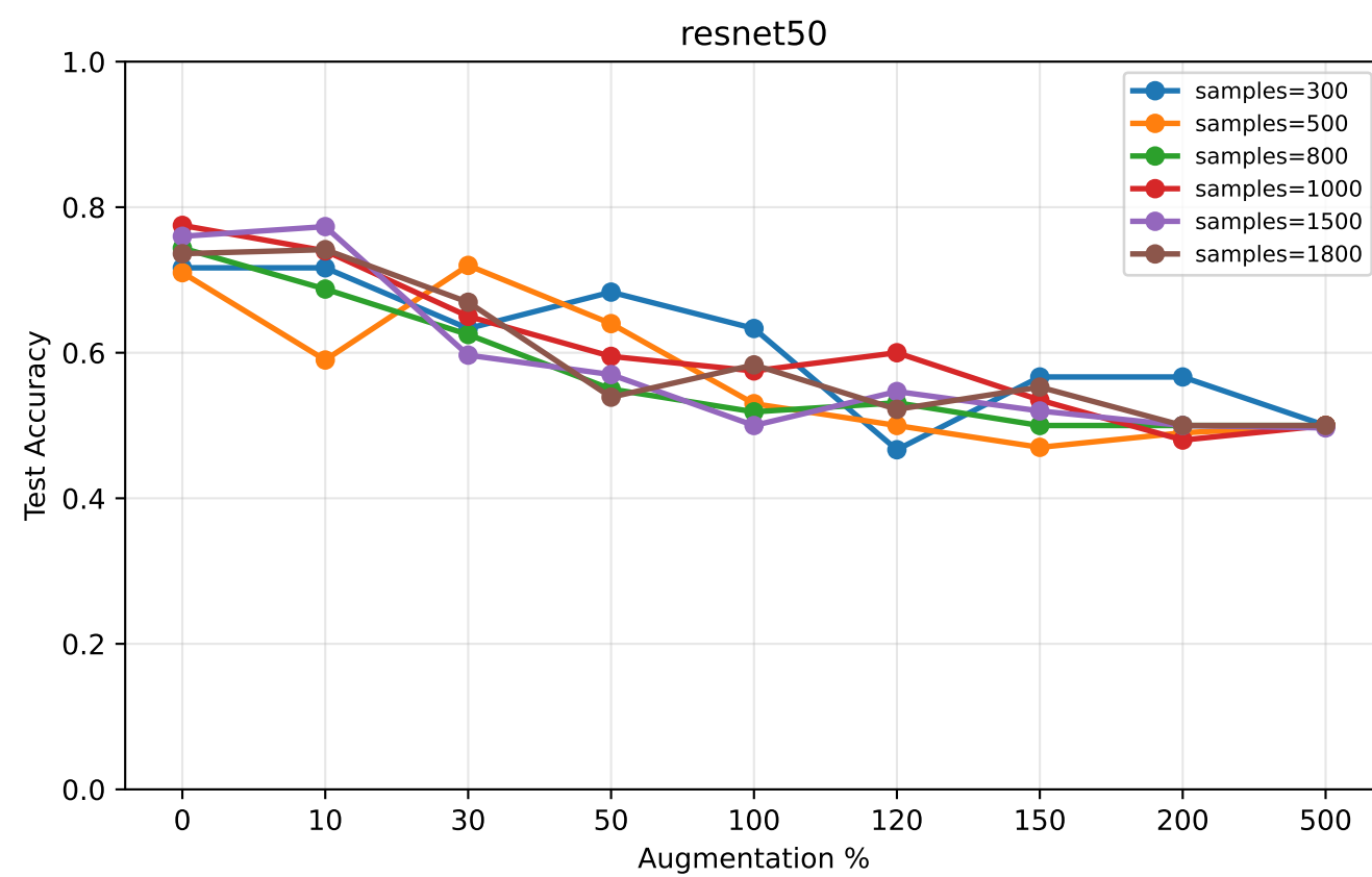
Accuracy vs Augmentation — withoutgap
