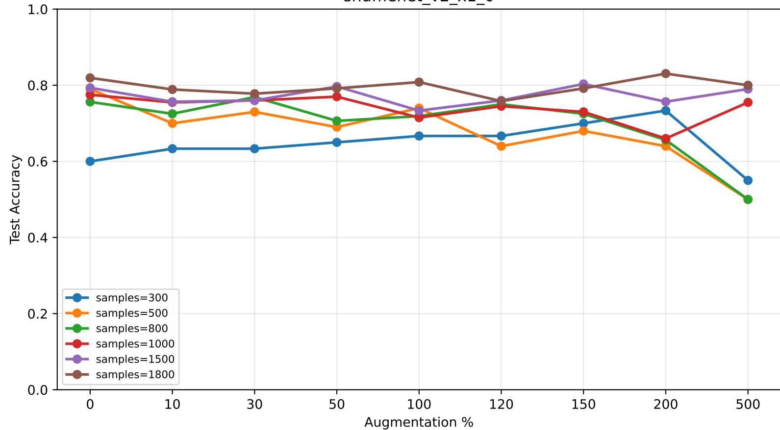
shufflenet_v2_x1_0
