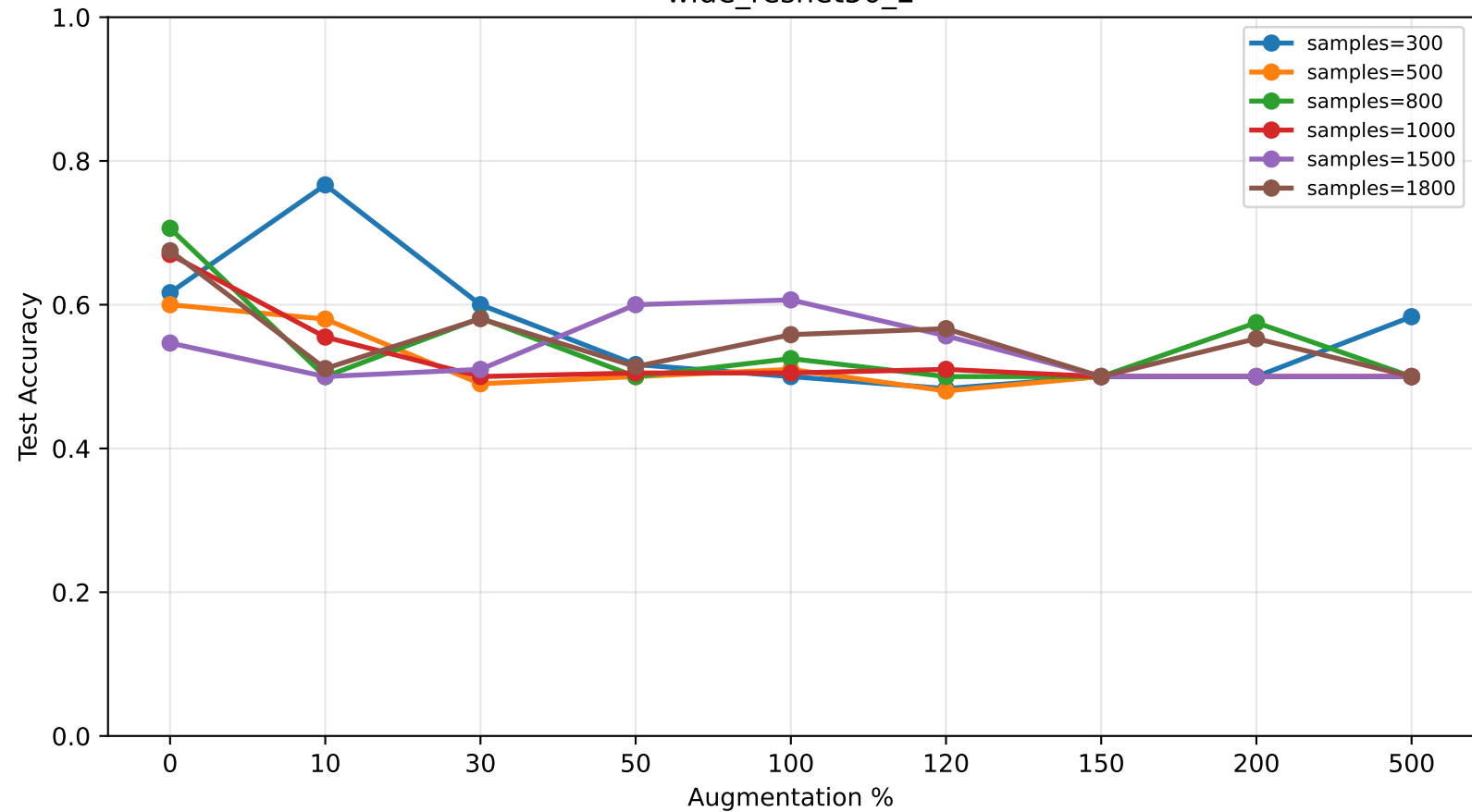
wide_resnet50_2
