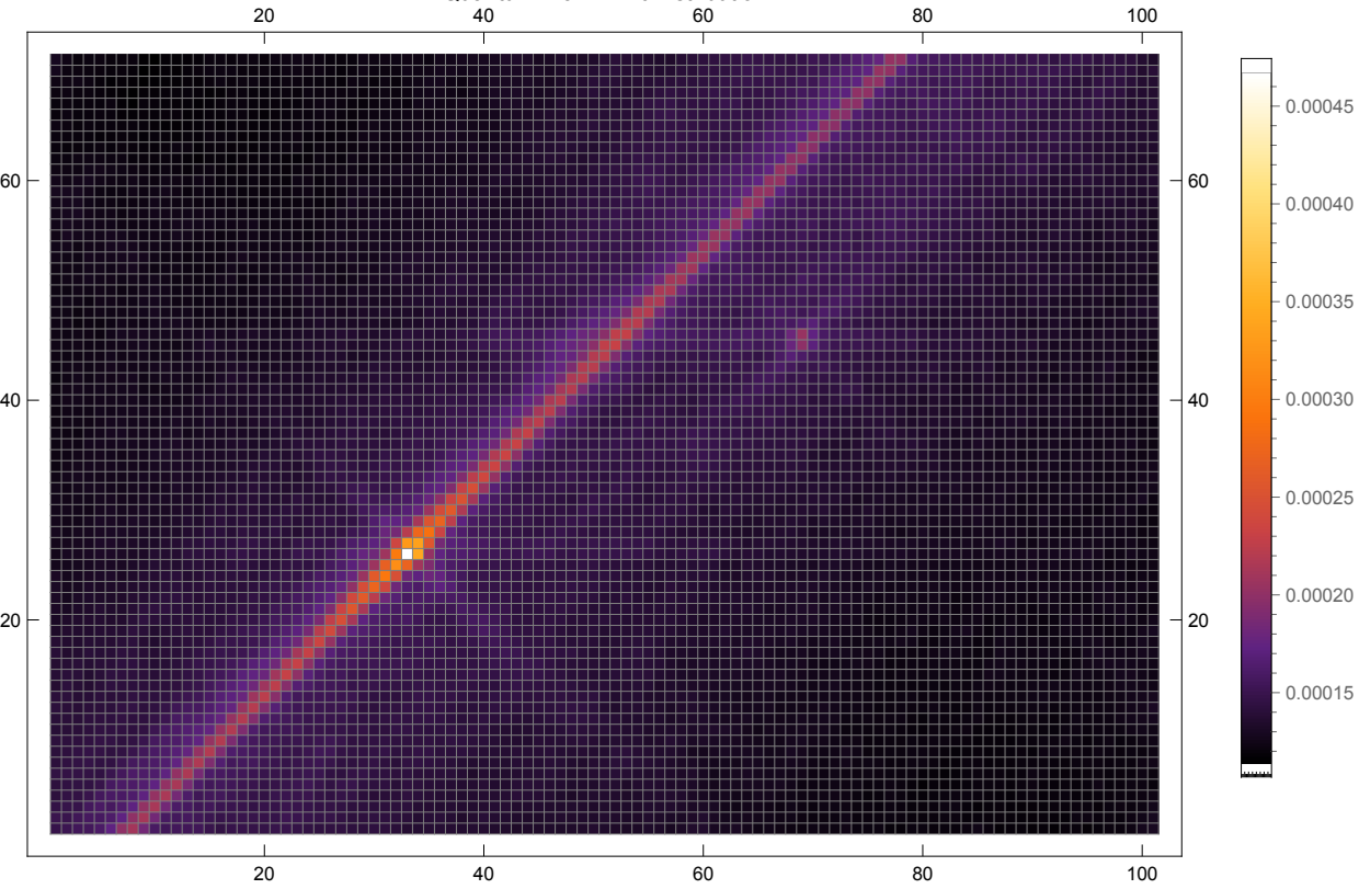
Quantum Walk Limit Distribution
