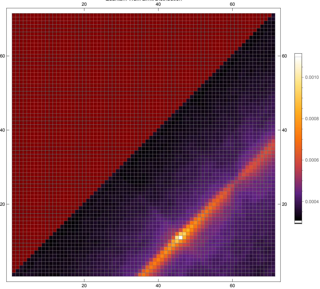
Quantum Walk Limit Distribution
