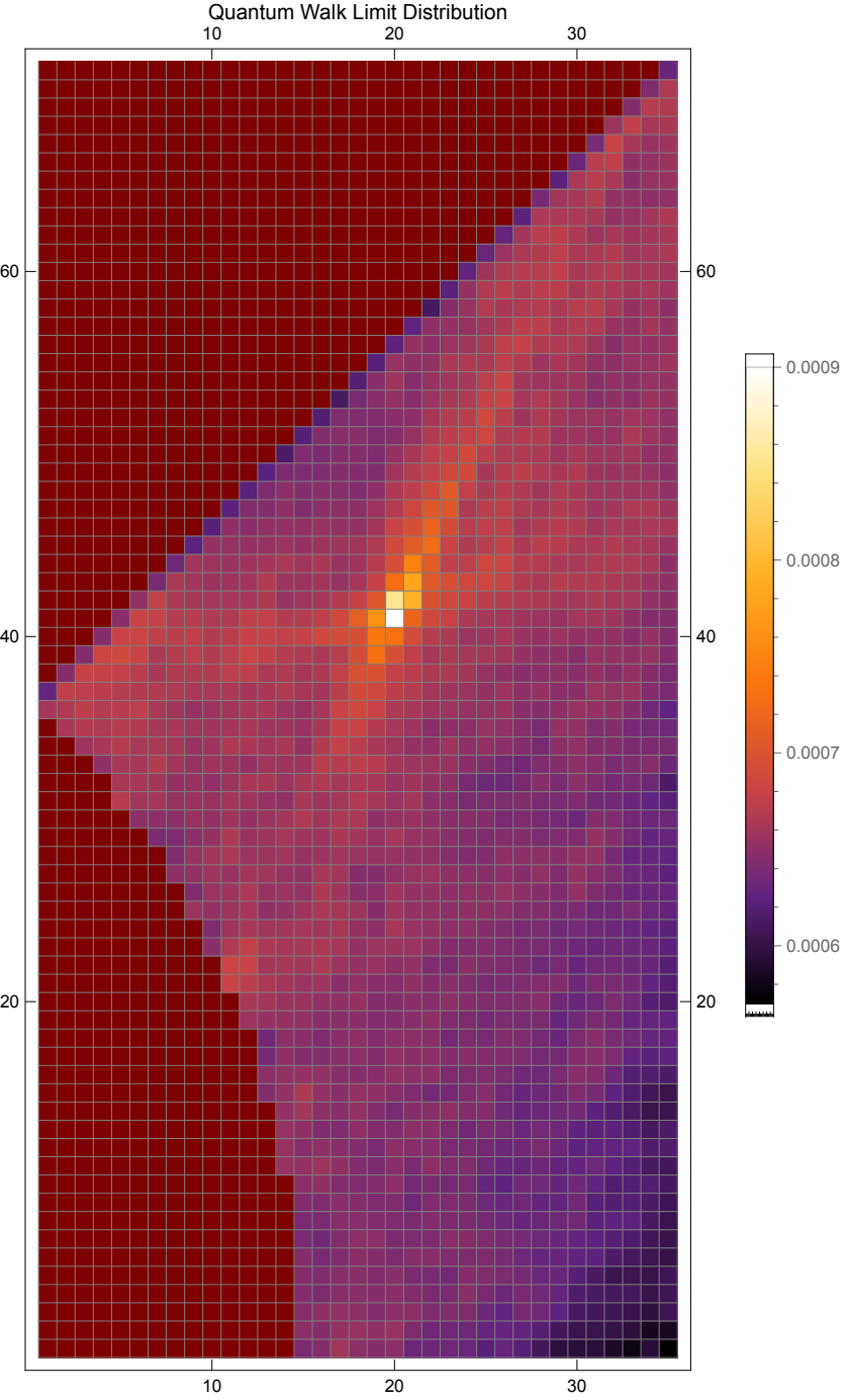
Quantum Walk Limit Distribution
