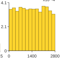
Unfold \times 10^{-4}
