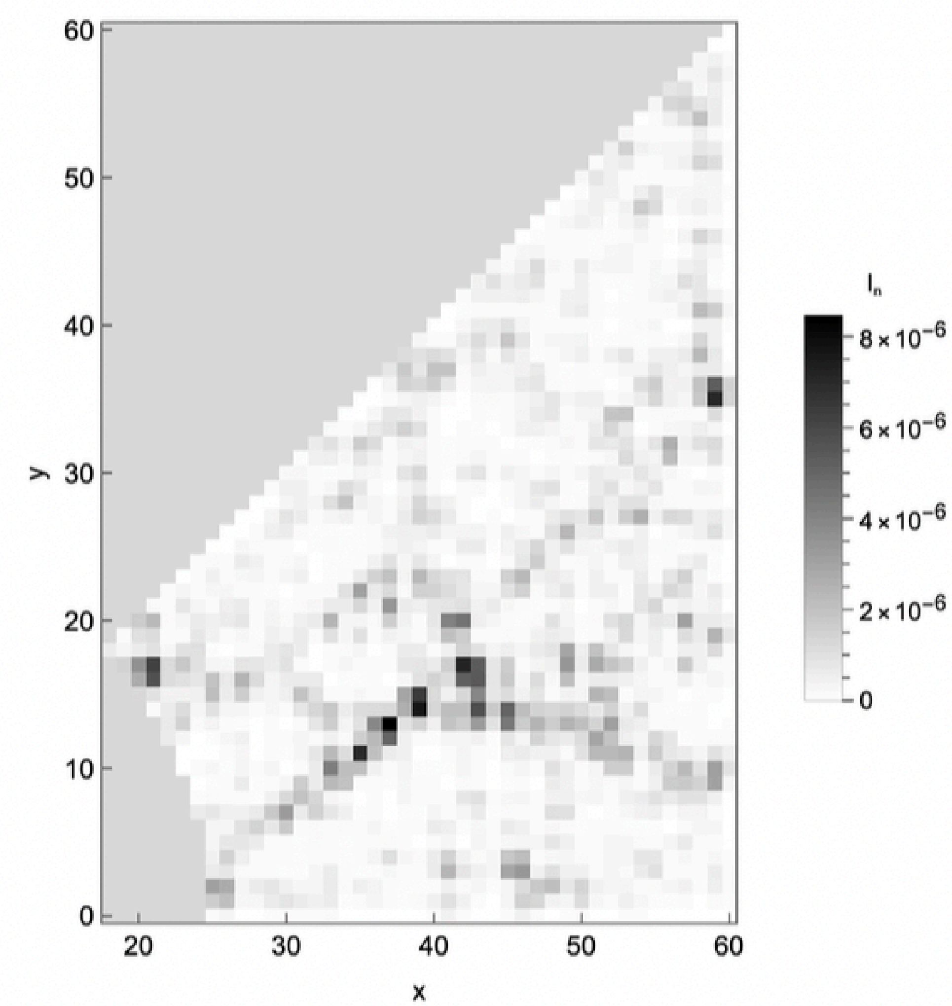
Intervalo 1: -3.14 a -2.36 \varepsilon = -2.7488 IPR = 8.89 \times 10^{-4} Residuo = 3.3 \times 10^{-14}
