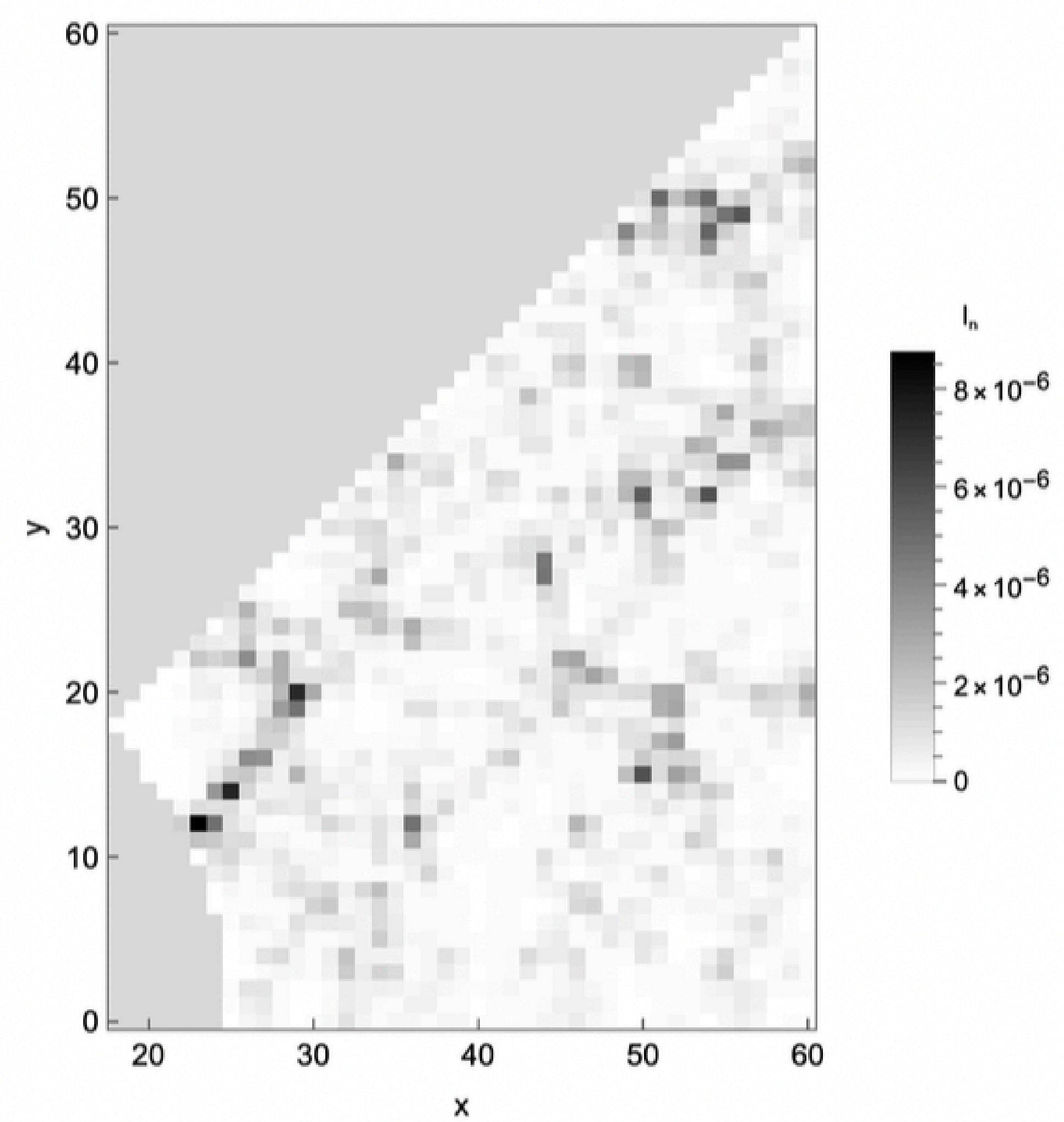
Intervalo 3: -1.57 a -0.79 \varepsilon = -1.1783 IPR = 8.84 \times 10^{-4} Residuo = 6.1 \times 10^{-14}
