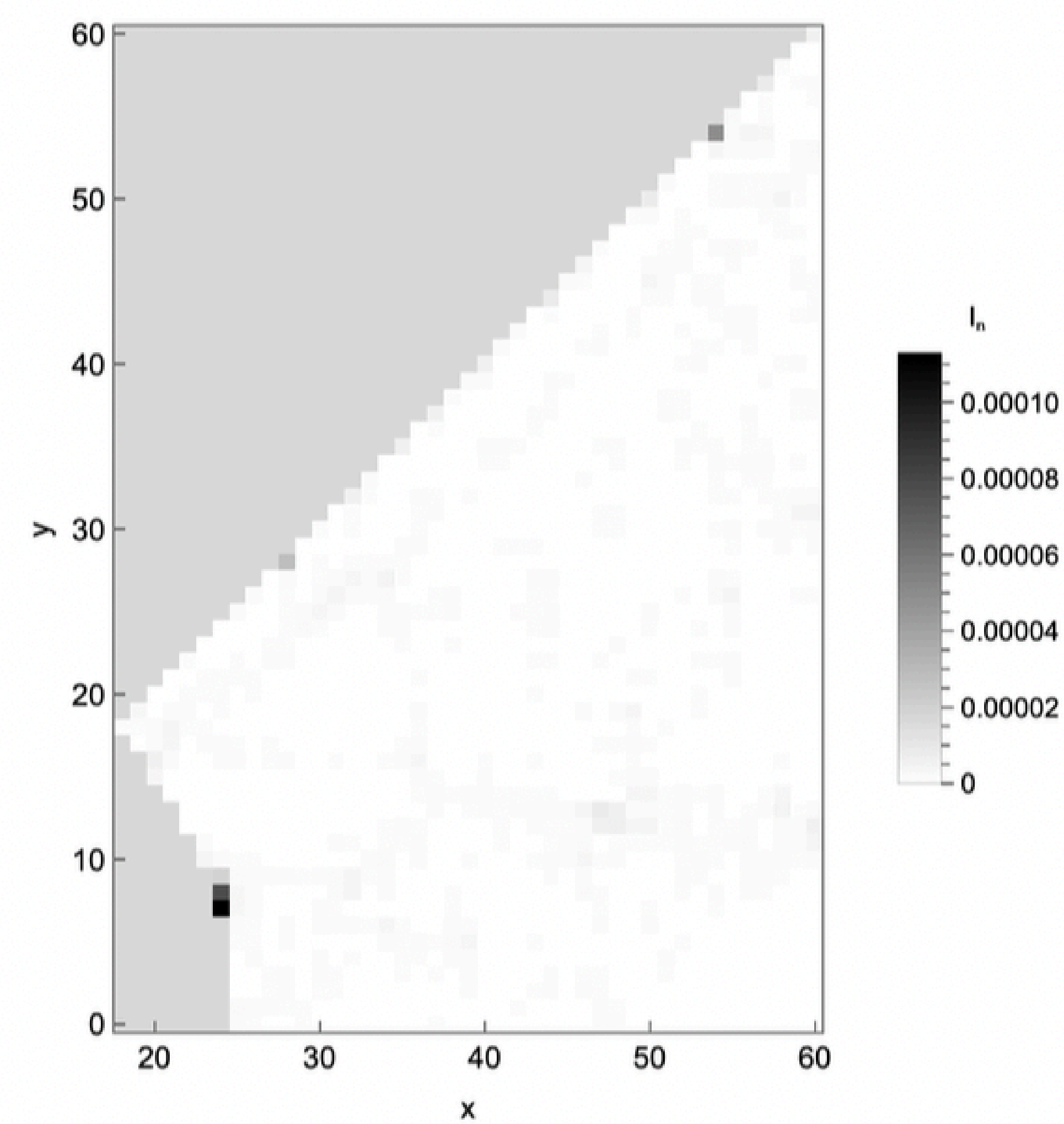
Intervalo 5: 0.00 a 0.79 \varepsilon = 0.3934 IPR = 1.14 \times 10^{-3} Residuo = 5. \times 10^{-14}
