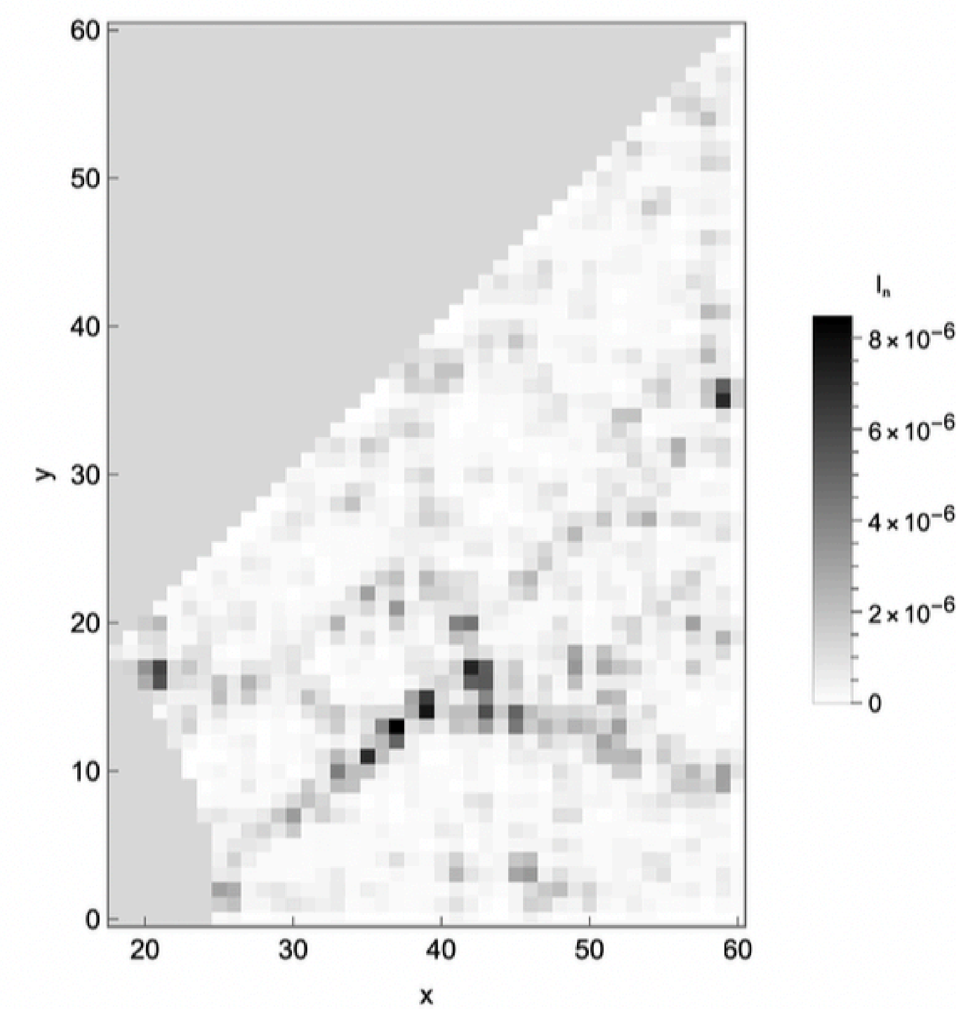
Intervalo 8: 2.36 a 3.14 \varepsilon = 2.7488 IPR = 8.89 \times 10^{-4} Residuo = 3.3 \times 10^{-14}
