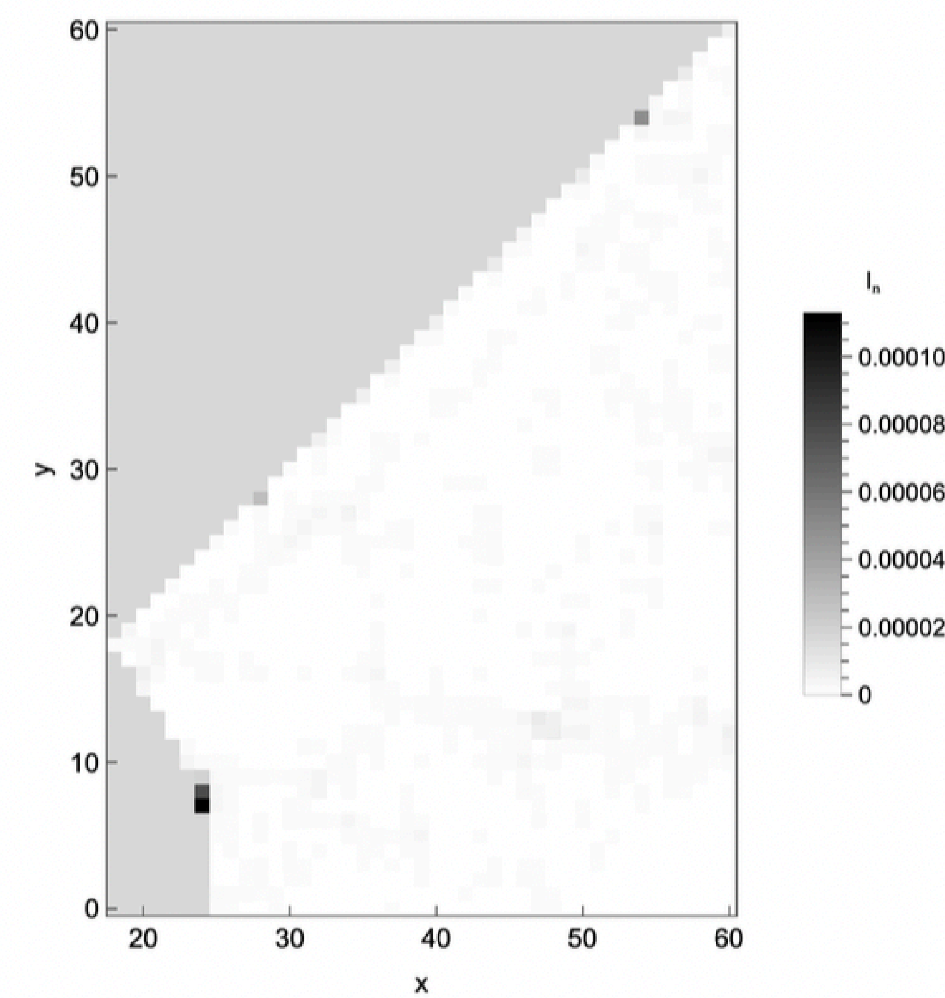
Intervalo 4: -0.79 a 0.00 \varepsilon = -0.3934 IPR = 1.14 \times 10^{-3} Residuo = 5. \times 10^{-14}
