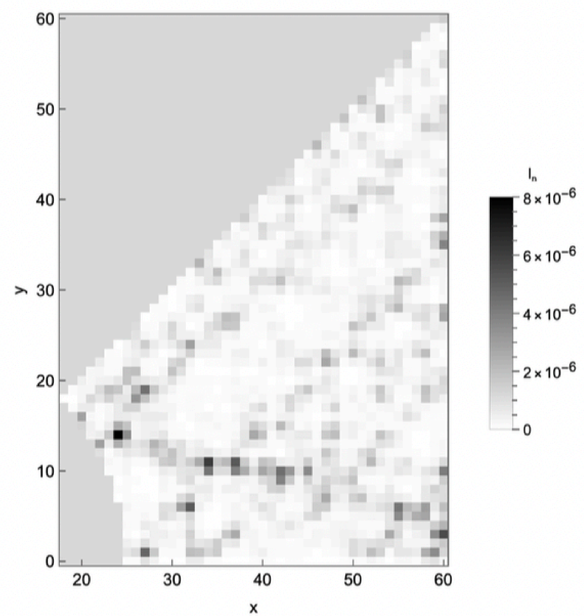
Intervalo 7: 1.57 a 2.36 \varepsilon = 1.9633 IPR = 8.5 \times 10^{-4} Residuo = 1.2 \times 10^{-13}
