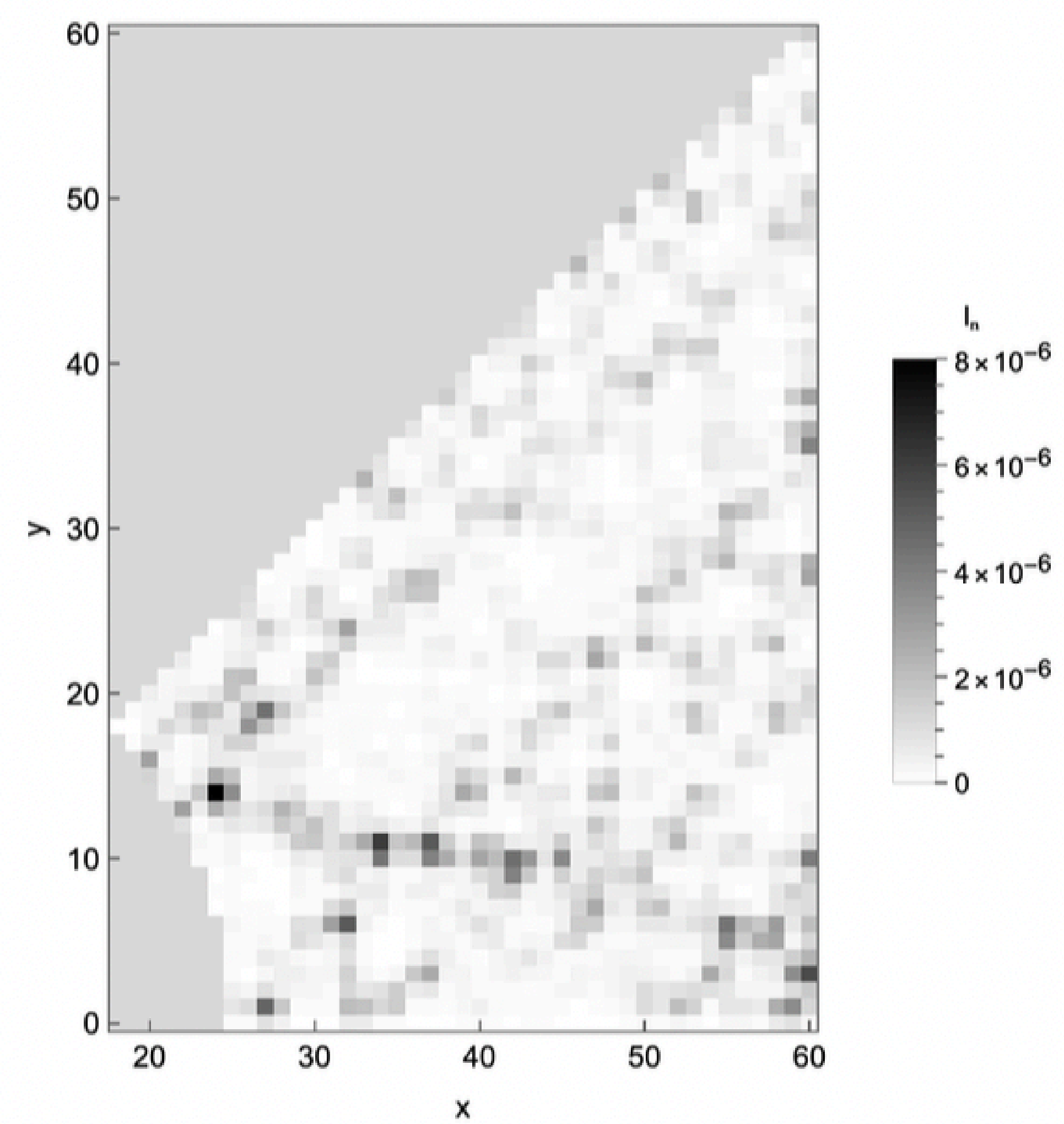
Intervalo 2: -2.36 a -1.57 \varepsilon = -1.9633 IPR = 8.5 \times 10^{-4} Residuo = 1.2 \times 10^{-13}
