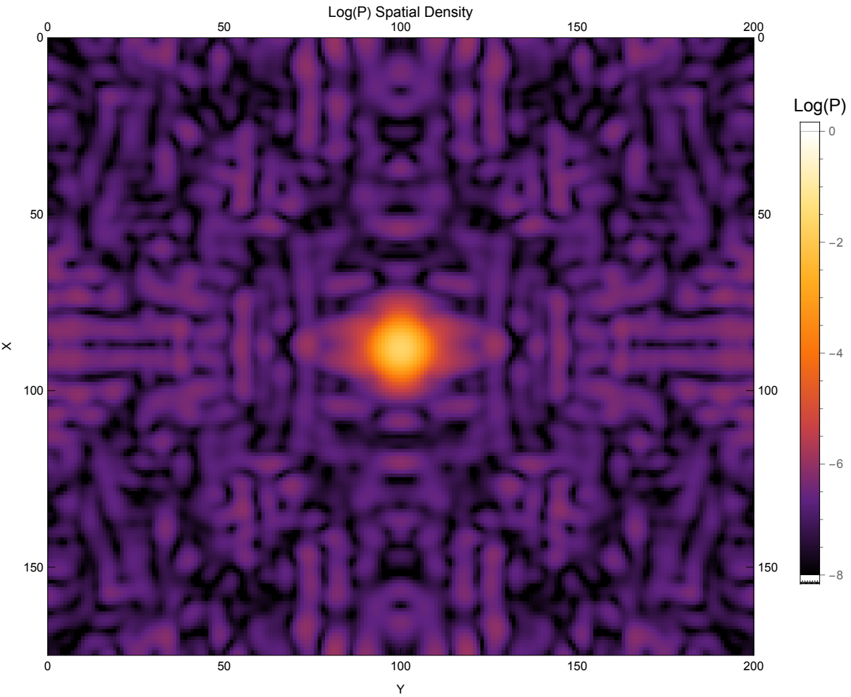
4D Grover State Morphology after t = 2275
