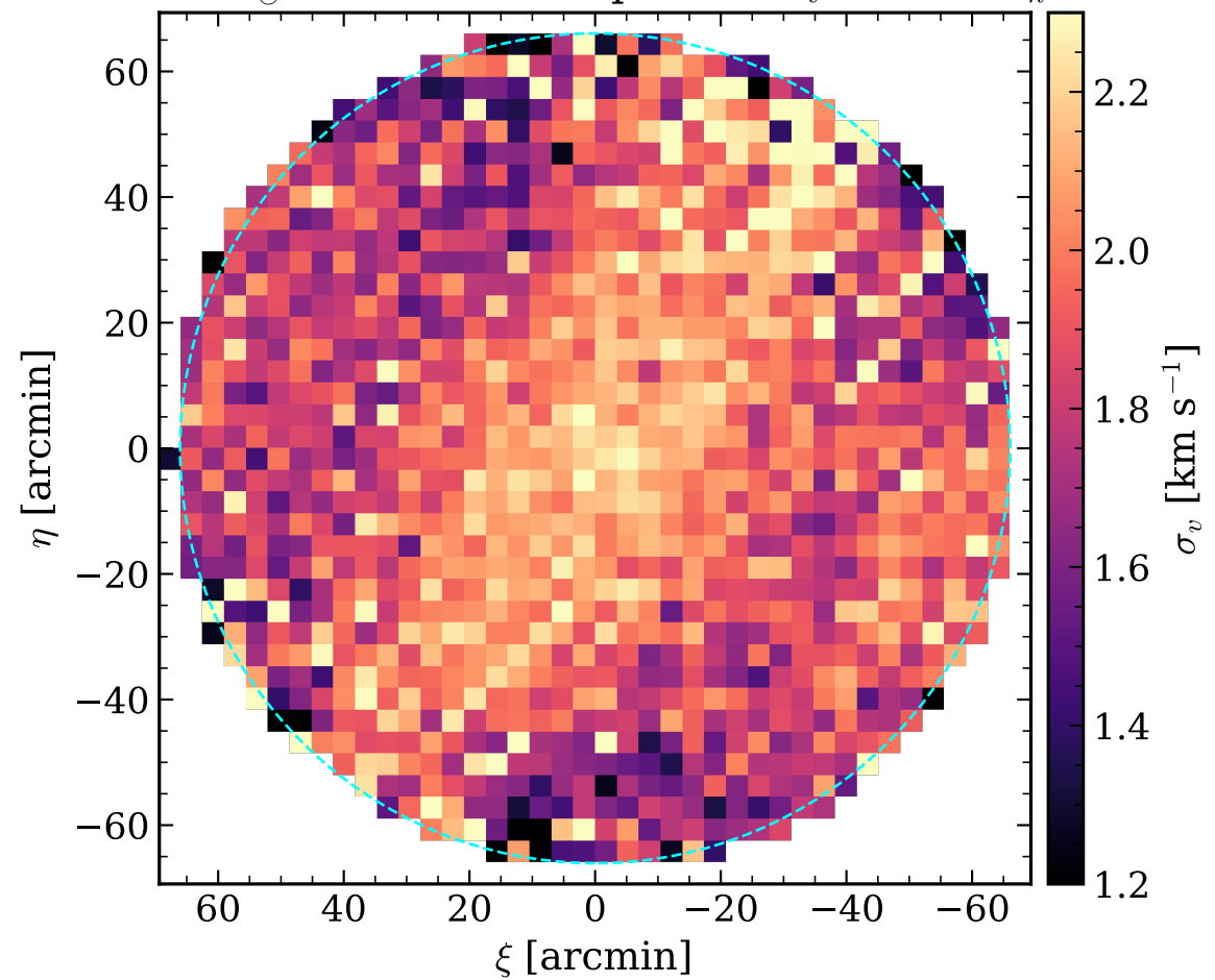
10 6 M ⊙ sim - LOSV dispersion \sigma_v within 2r_h
