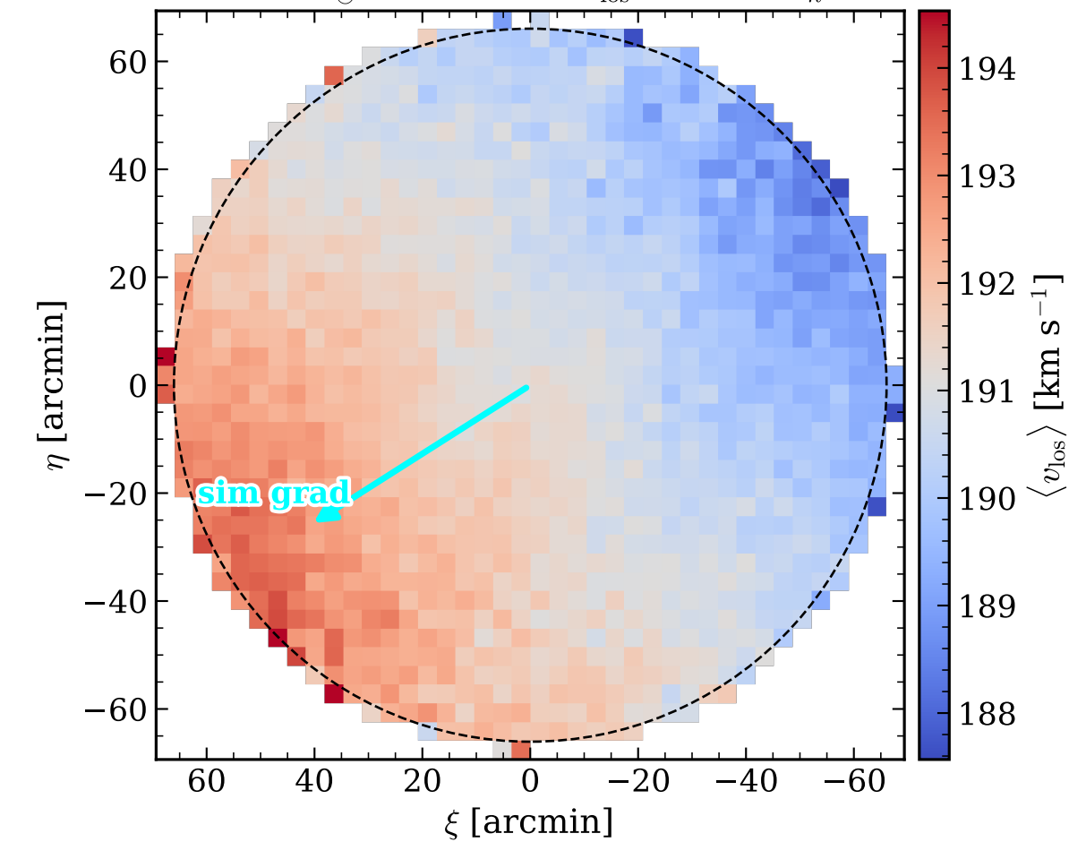
10 6 M ⊙ sim - mean v_{\text{los}} within 2r_h
